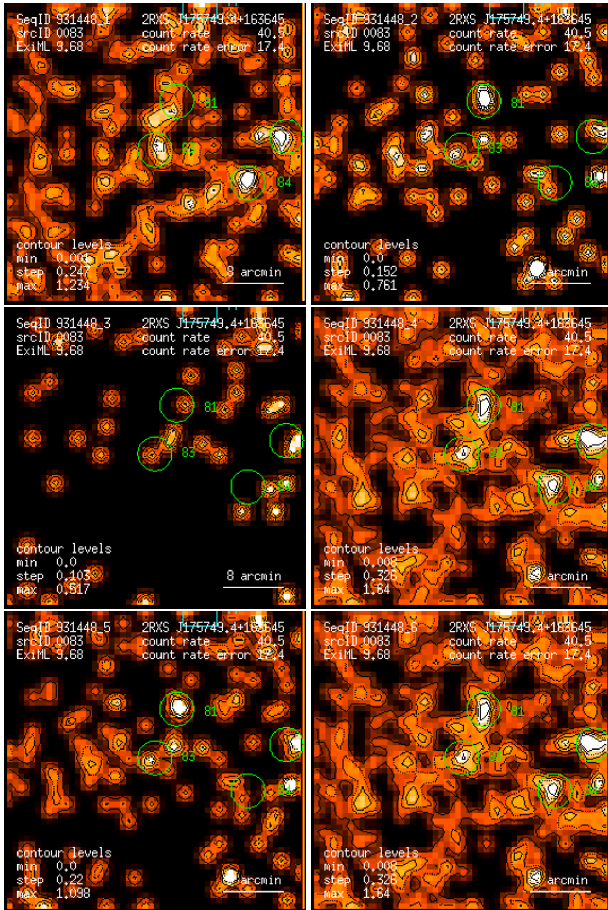
Figure 83: RASS 931448: detection 0083: band rate images, Gaussian filter: (1) PSPC channels 11 – 41, (2) 52 – 90, (3) 91 – 201, (4) 11 – 235, (5) 52 – 201, (6) 11 – 201. Broad band rates in counts/ks. Band rate contour levels in counts/ks/arcmin 2 .
