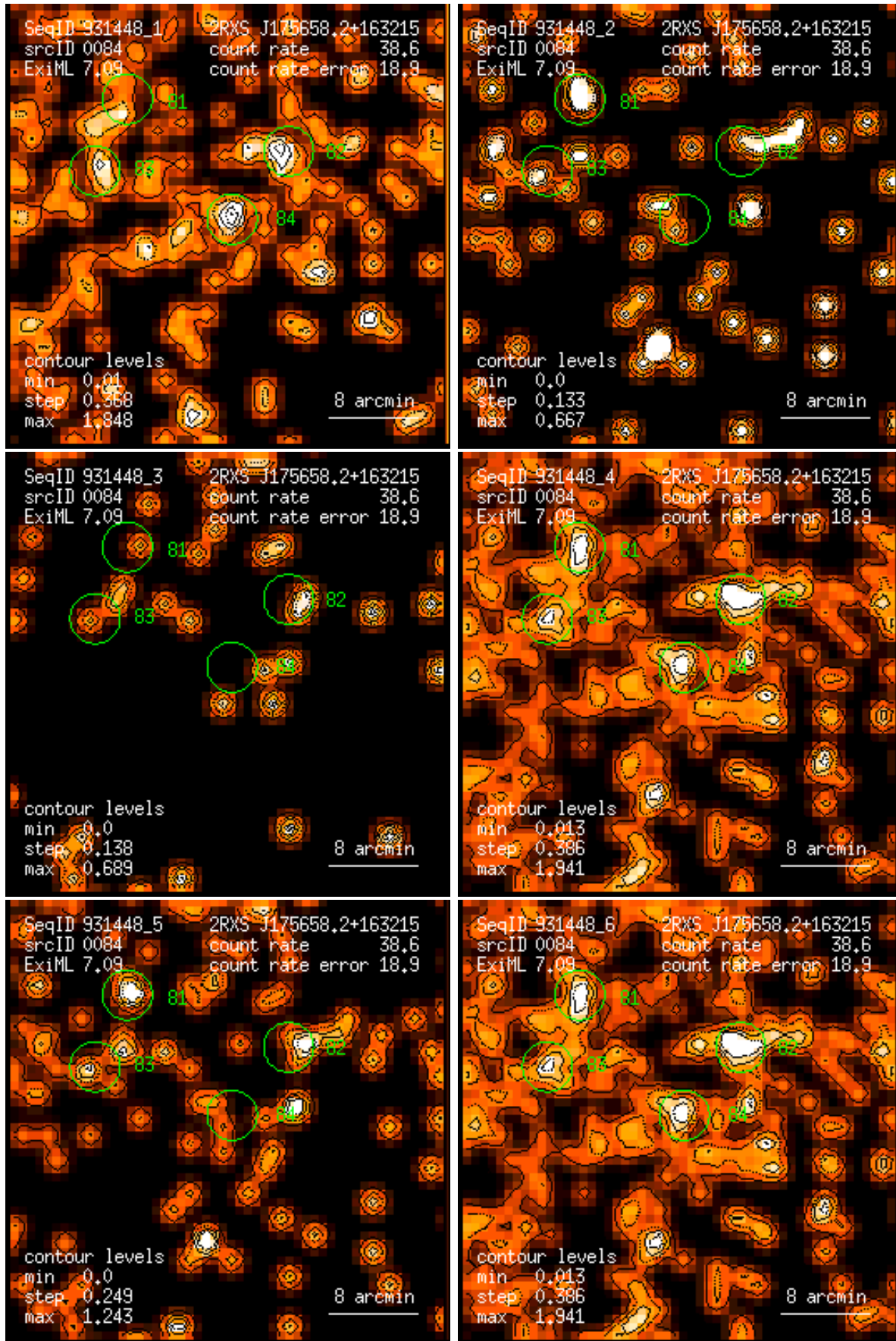
Figure 84: RASS 931448: detection 0084: band rate images, Gaussian filter: (1) PSPC channels 11 – 41, (2) 52 – 90, (3) 91 – 201, (4) 11 – 235, (5) 52 – 201, (6) 11 – 201. Broad band rates in counts/ks. Band rate contour levels in counts/ks/arcmin 2 .
