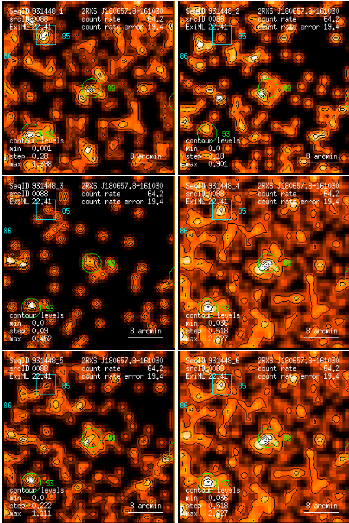
Figure 88: RASS 931448: detection 0088: band rate images, Gaussian filter: (1) PSPC channels 11 – 41, (2) 52 – 90, (3) 91 – 201, (4) 11 – 235, (5) 52 – 201, (6) 11 – 201. Broad band rates in counts/ks. Band rate contour levels in counts/ks/arcmin 2 .
