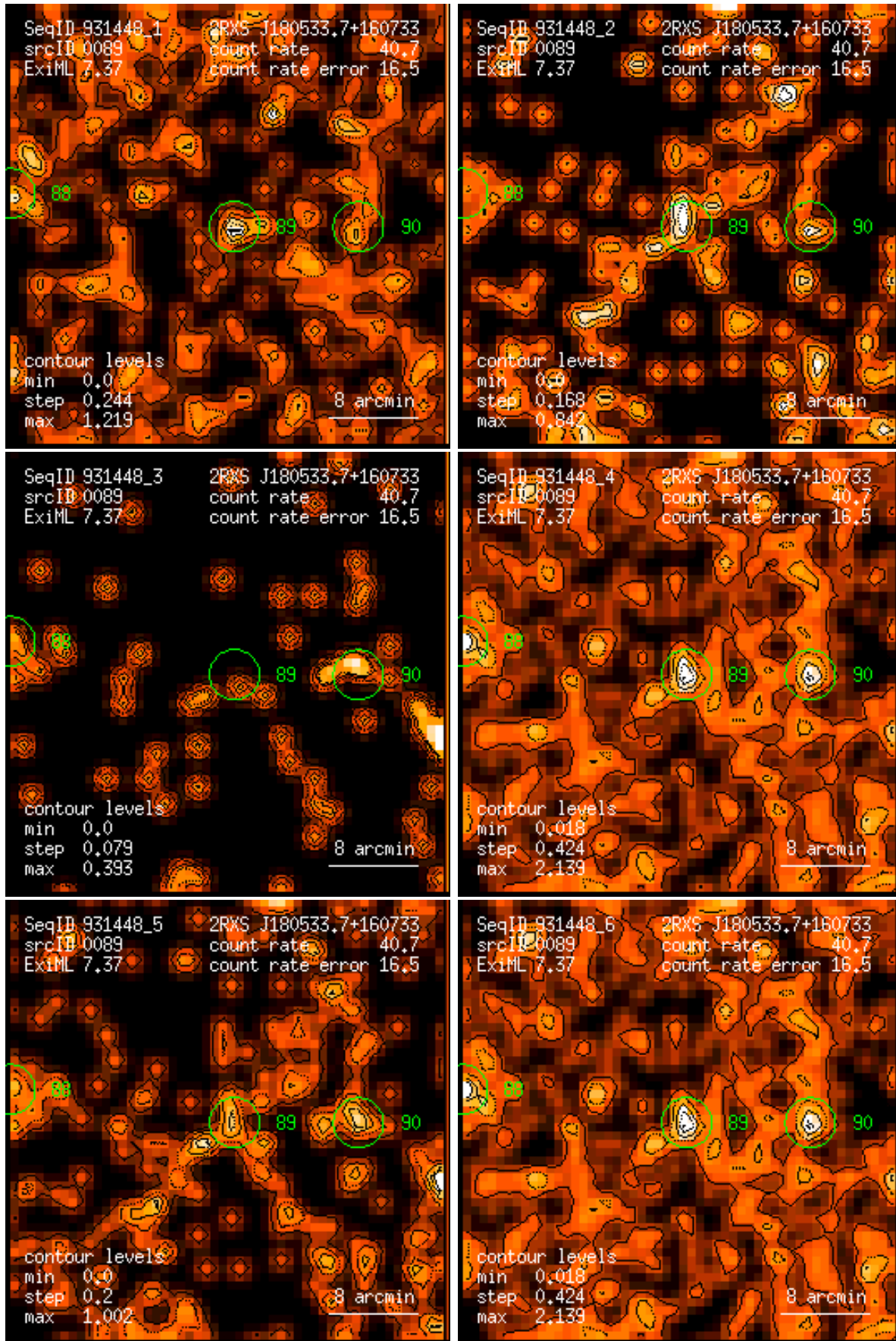
Figure 89: RASS 931448: detection 0089: band rate images, Gaussian filter: (1) PSPC channels 11 – 41, (2) 52 – 90, (3) 91 – 201, (4) 11 – 235, (5) 52 – 201, (6) 11 – 201. Broad band rates in counts/ks. Band rate contour levels in counts/ks/arcmin 2 .
