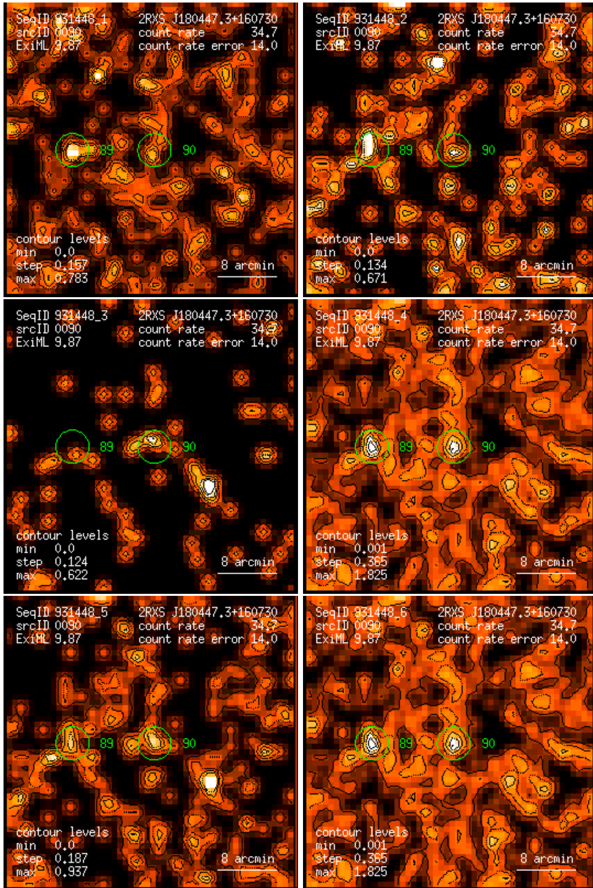
Figure 90: RASS 931448: detection 0090: band rate images, Gaussian filter: (1) PSPC channels 11 – 41, (2) 52 – 90, (3) 91 – 201, (4) 11 – 235, (5) 52 – 201, (6) 11 – 201. Broad band rates in counts/ks. Band rate contour levels in counts/ks/arcmin 2 .
