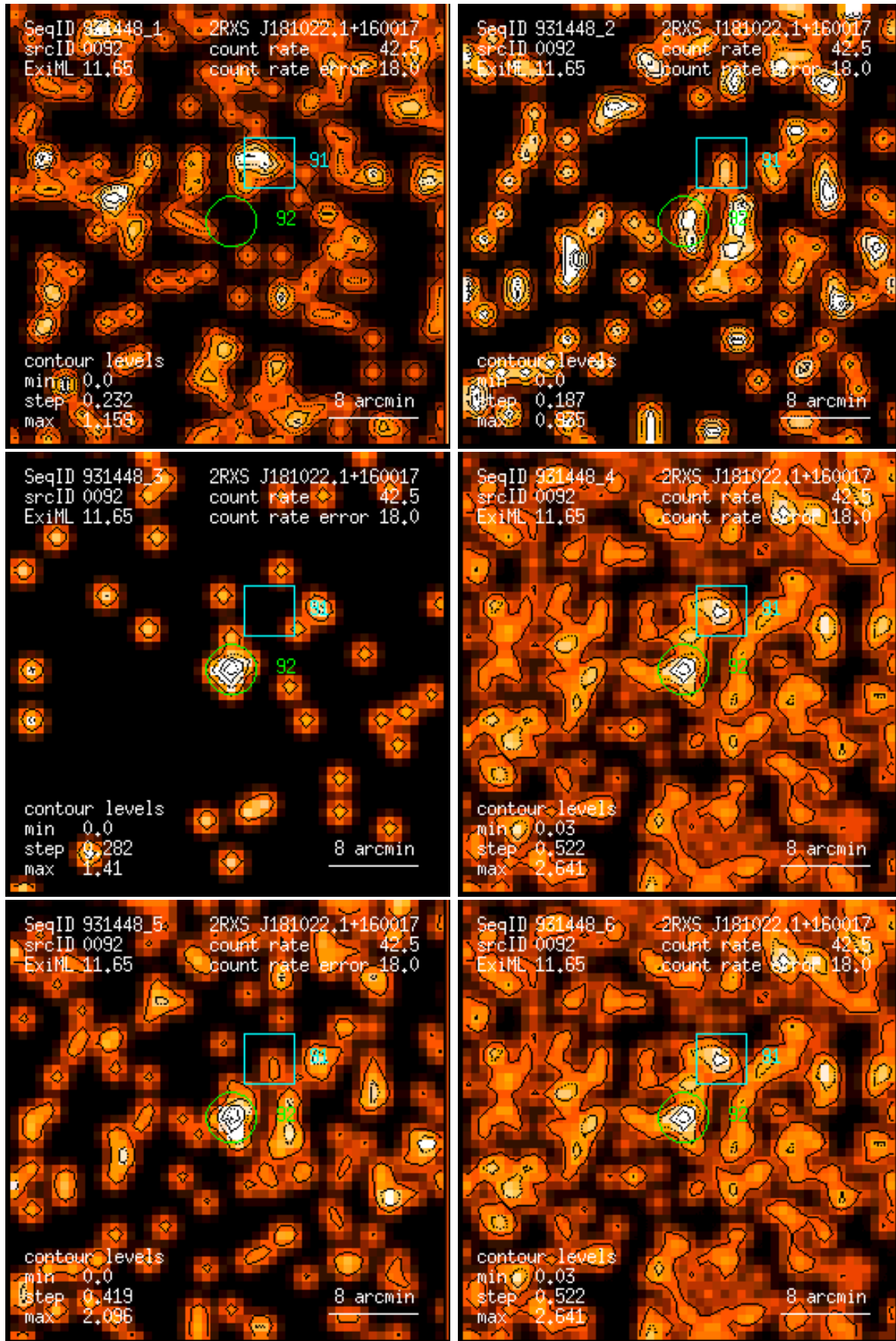
Figure 92: RASS 931448: detection 0092: band rate images, Gaussian filter: (1) PSPC channels 11 – 41, (2) 52 – 90, (3) 91 – 201, (4) 11 – 235, (5) 52 – 201, (6) 11 – 201. Broad band rates in counts/ks. Band rate contour levels in counts/ks/arcmin 2 .
