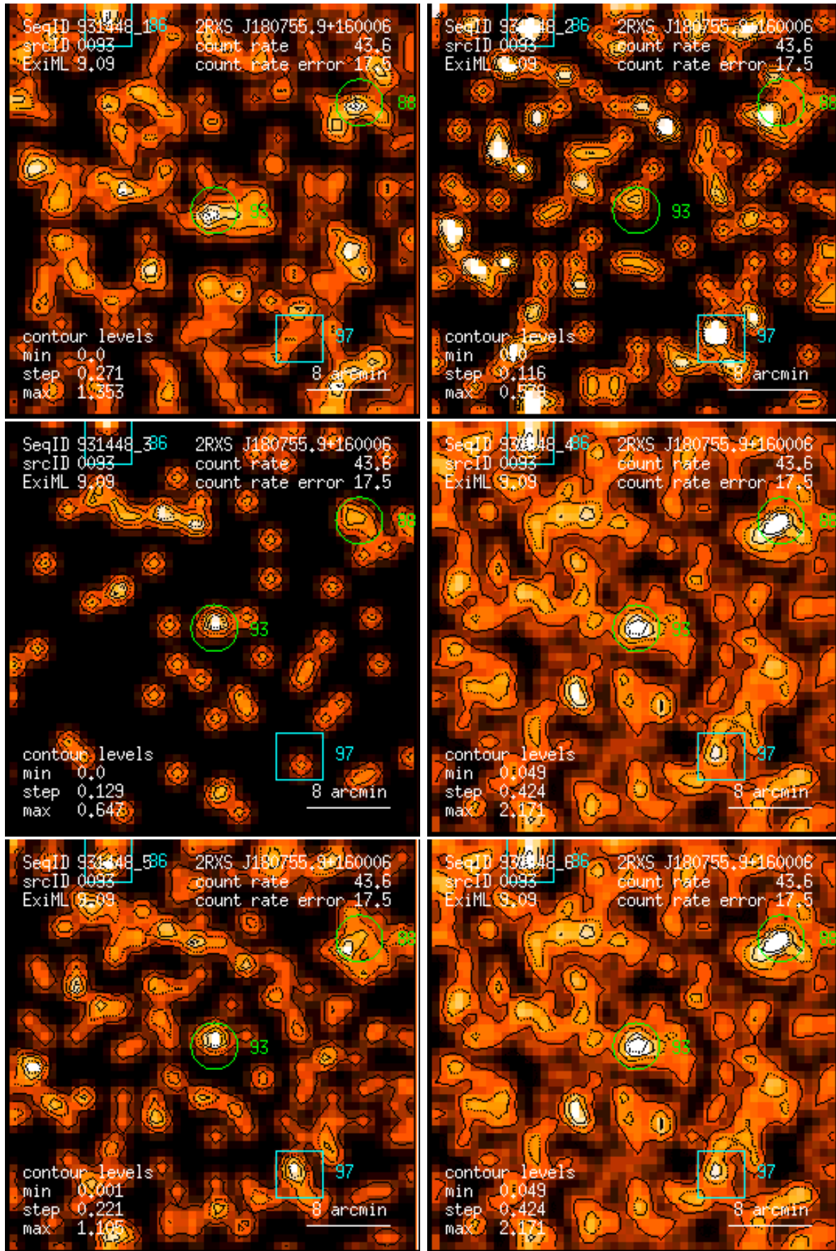
Figure 93: RASS 931448: detection 0093: band rate images, Gaussian filter: (1) PSPC channels 11 – 41, (2) 52 – 90, (3) 91 – 201, (4) 11 – 235, (5) 52 – 201, (6) 11 – 201. Broad band rates in counts/ks. Band rate contour levels in counts/ks/arcmin 2 .
