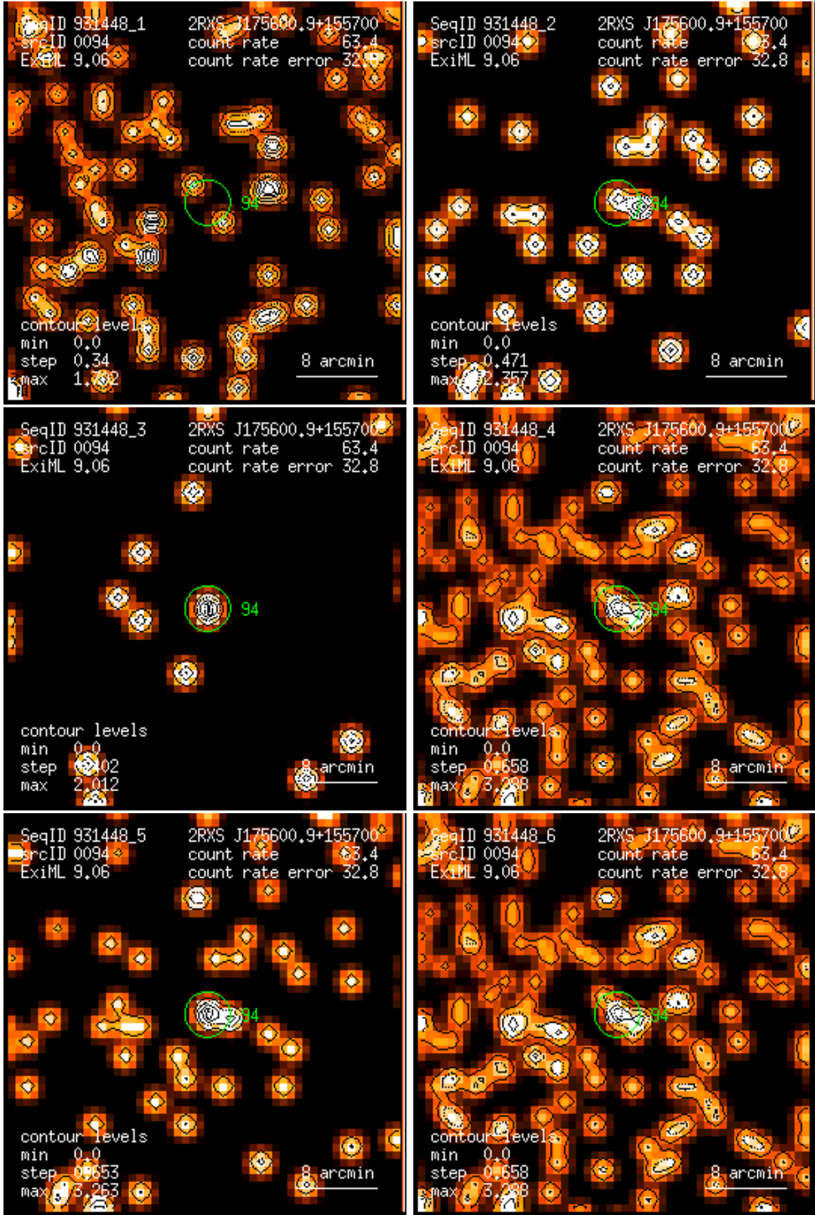
Figure 94: RASS 931448: detection 0094: band rate images, Gaussian filter: (1) PSPC channels 11 – 41, (2) 52 – 90, (3) 91 – 201, (4) 11 – 235, (5) 52 – 201, (6) 11 – 201. Broad band rates in counts/ks. Band rate contour levels in counts/ks/arcmin 2 .
