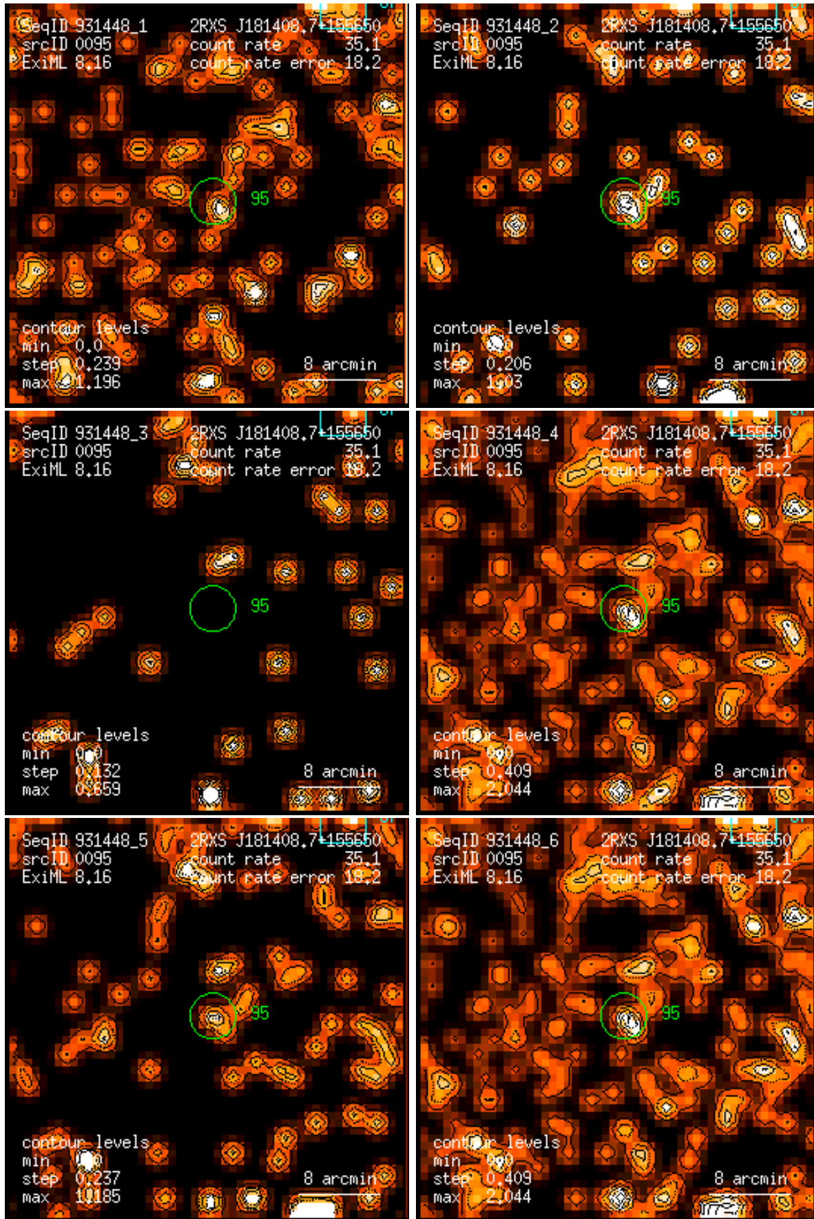
Figure 95: RASS 931448: detection 0095: band rate images, Gaussian filter: (1) PSPC channels 11 – 41, (2) 52 – 90, (3) 91 – 201, (4) 11 – 235, (5) 52 – 201, (6) 11 – 201. Broad band rates in counts/ks. Band rate contour levels in counts/ks/arcmin 2 .
