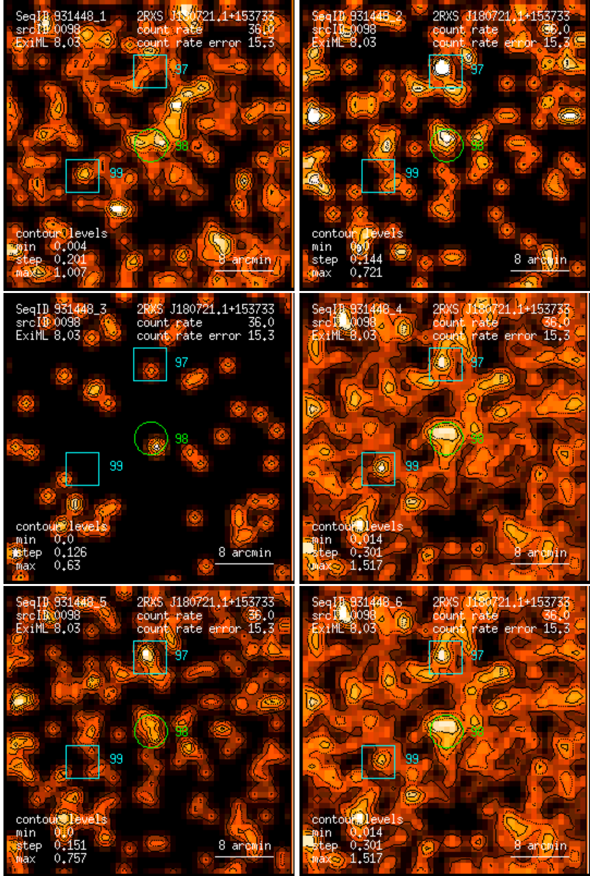
Figure 98: RASS 931448: detection 0098: band rate images, Gaussian filter: (1) PSPC channels 11 – 41, (2) 52 – 90, (3) 91 – 201, (4) 11 – 235, (5) 52 – 201, (6) 11 – 201. Broad band rates in counts/ks. Band rate contour levels in counts/ks/arcmin 2 .
