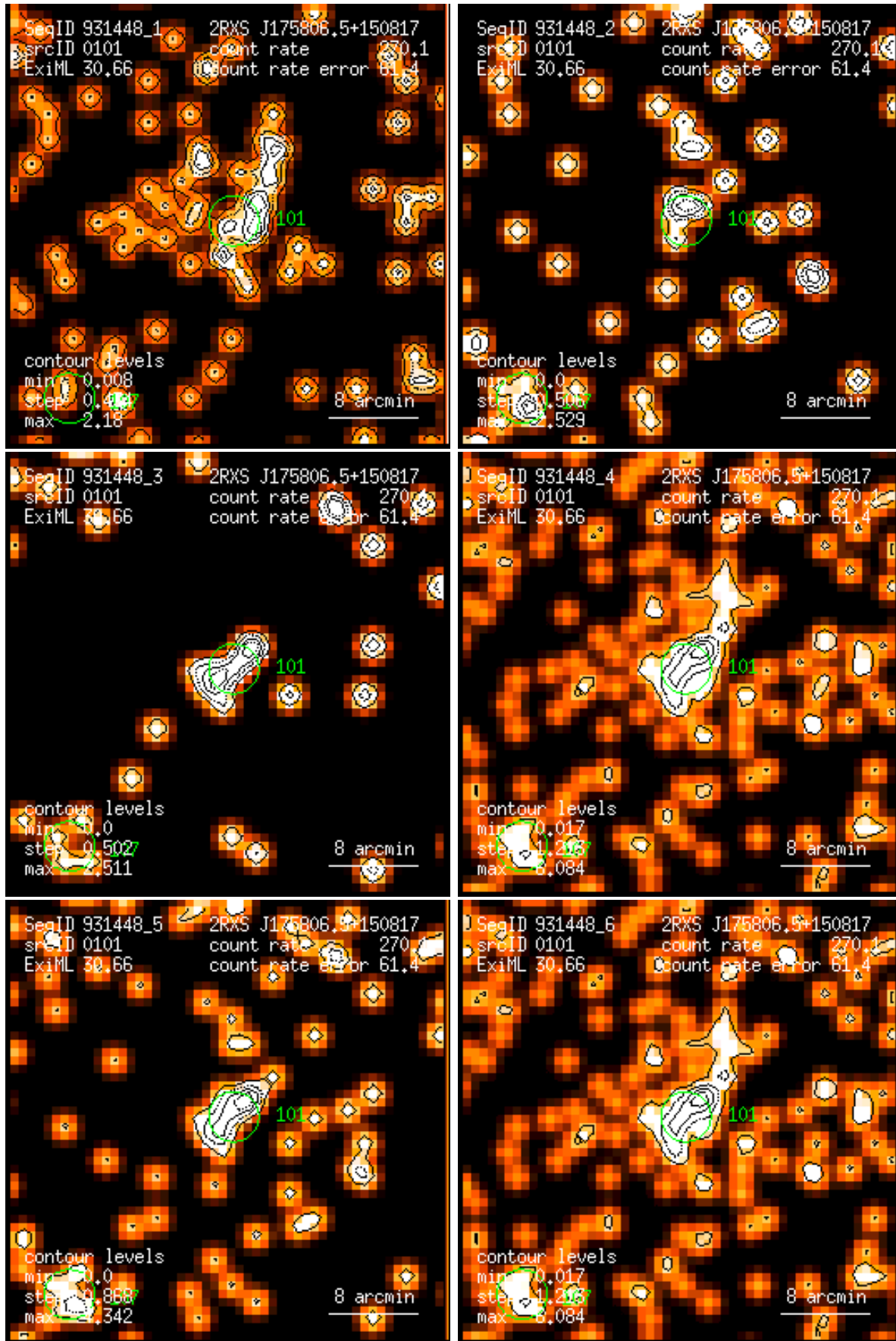
Figure 101: RASS 931448: detection 0101: band rate images, Gaussian filter: (1) PSPC channels 11 – 41, (2) 52 – 90, (3) 91 – 201, (4) 11 – 235, (5) 52 – 201, (6) 11 – 201. Broad band rates in counts/ks. Band rate contour levels in counts/ks/arcmin 2 .
