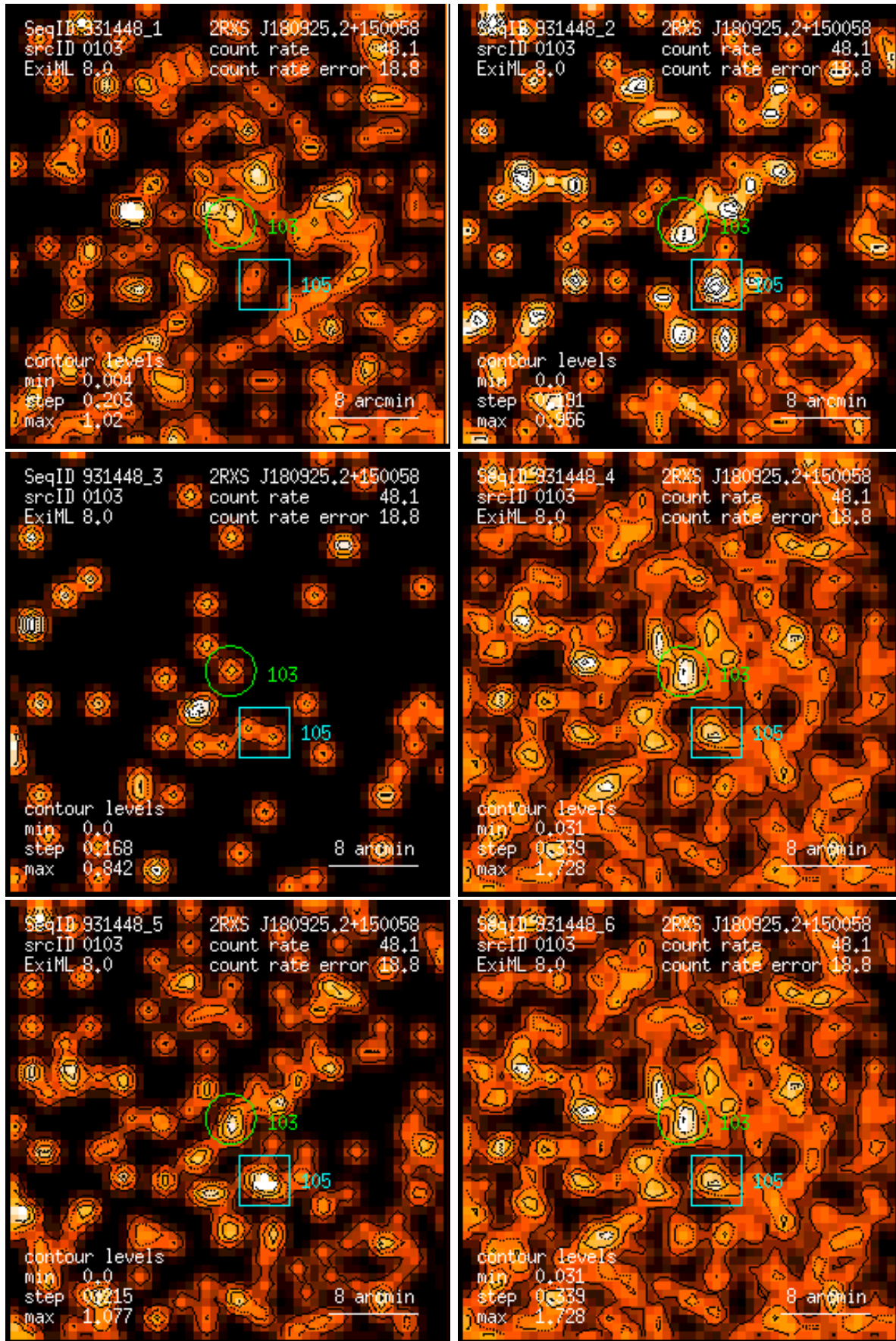
Figure 103: RASS 931448: detection 0103: band rate images, Gaussian filter: (1) PSPC channels 11 – 41, (2) 52 – 90, (3) 91 – 201, (4) 11 – 235, (5) 52 – 201, (6) 11 – 201. Broad band rates in counts/ks. Band rate contour levels in counts/ks/arcmin 2 .
