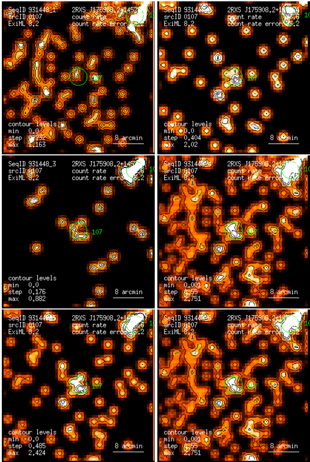
Figure 107: RASS 931448: detection 0107: band rate images, Gaussian filter: (1) PSPC channels 11 – 41, (2) 52 – 90, (3) 91 – 201, (4) 11 – 235, (5) 52 – 201, (6) 11 – 201. Broad band rates in counts/ks. Band rate contour levels in counts/ks/arcmin 2 .
