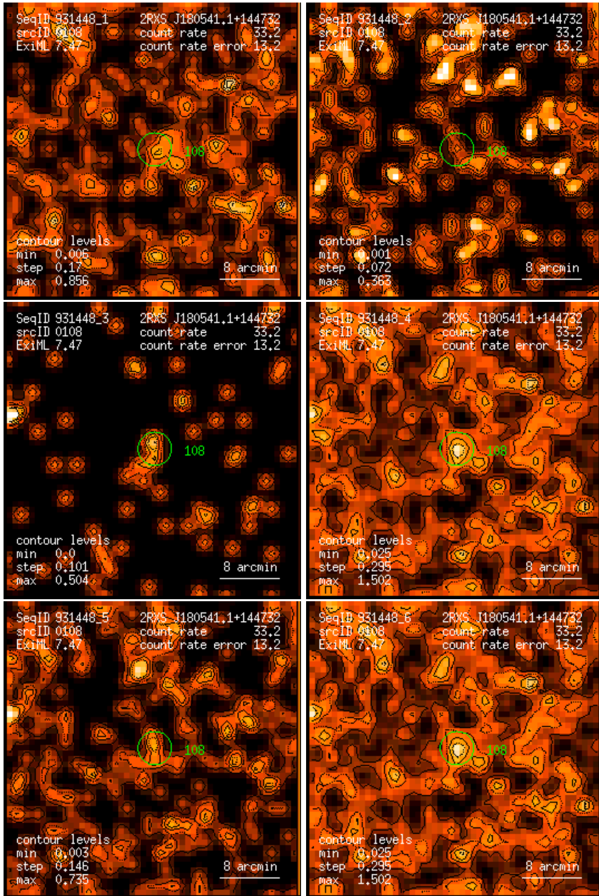
Figure 108: RASS 931448: detection 0108: band rate images, Gaussian filter: (1) PSPC channels 11 – 41, (2) 52 – 90, (3) 91 – 201, (4) 11 – 235, (5) 52 – 201, (6) 11 – 201. Broad band rates in counts/ks. Band rate contour levels in counts/ks/arcmin 2 .
