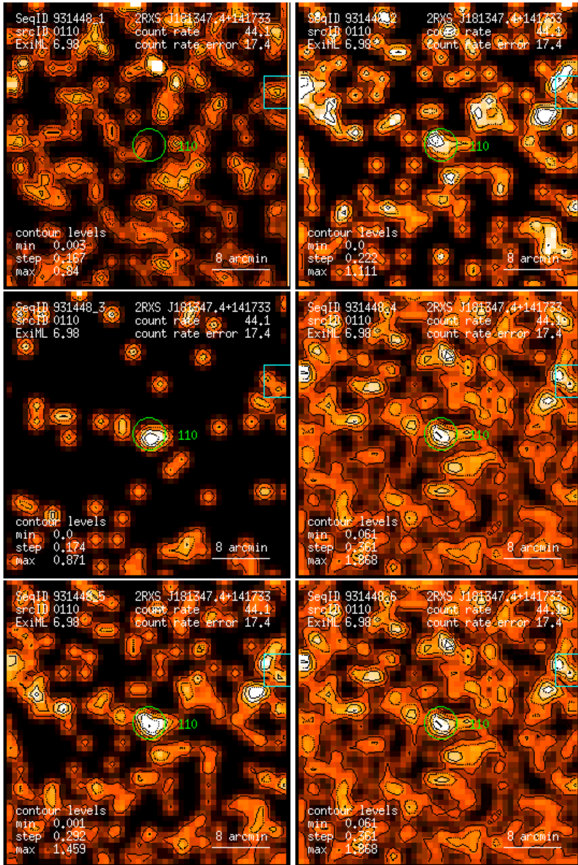
Figure 110: RASS 931448: detection 0110: band rate images, Gaussian filter: (1) PSPC channels 11 – 41, (2) 52 – 90, (3) 91 – 201, (4) 11 – 235, (5) 52 – 201, (6) 11 – 201. Broad band rates in counts/ks. Band rate contour levels in counts/ks/arcmin 2 .
