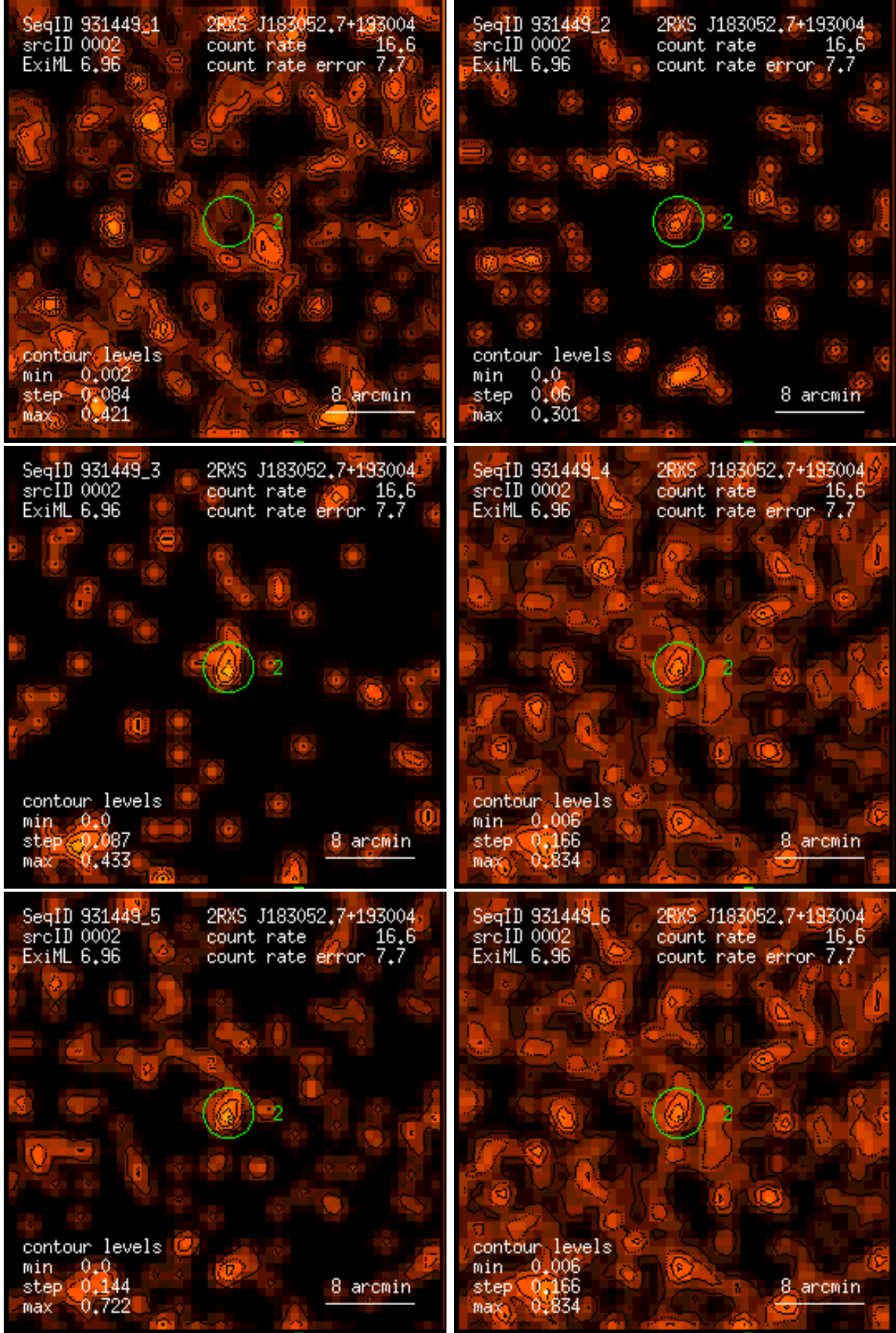
Figure 2: RASS 931449: detection 0002: band rate images, Gaussian filter: (1) PSPC channels 11 – 41, (2) 52 – 90, (3) 91 – 201, (4) 11 – 235, (5) 52 – 201, (6) 11 – 201. Broad band rates in counts/ks. Band rate contour levels in counts/ks/arcmin 2 .
