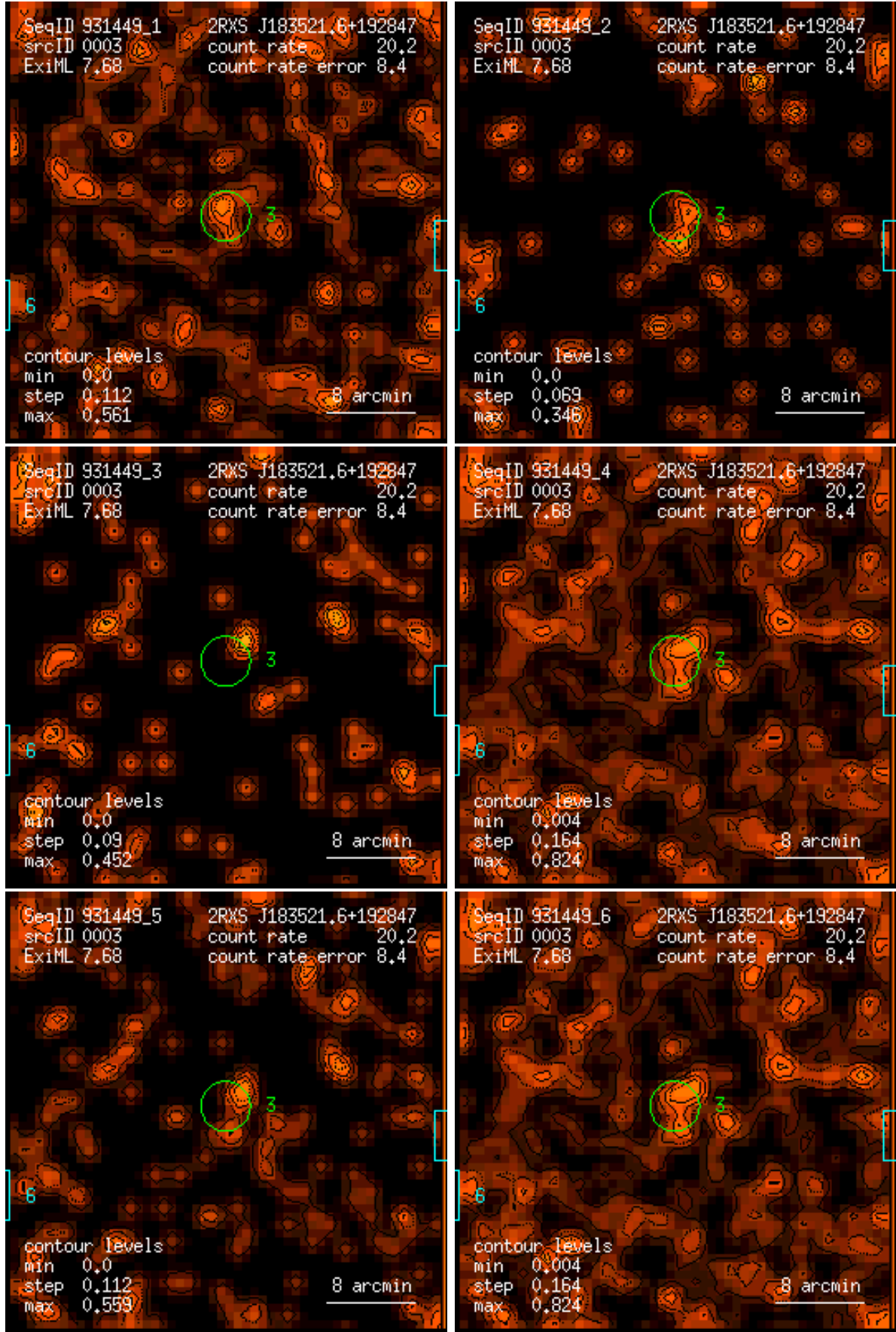
Figure 3: RASS 931449: detection 0003: band rate images, Gaussian filter: (1) PSPC channels 11 – 41, (2) 52 – 90, (3) 91 – 201, (4) 11 – 235, (5) 52 – 201, (6) 11 – 201. Broad band rates in counts/ks. Band rate contour levels in counts/ks/arcmin 2 .
