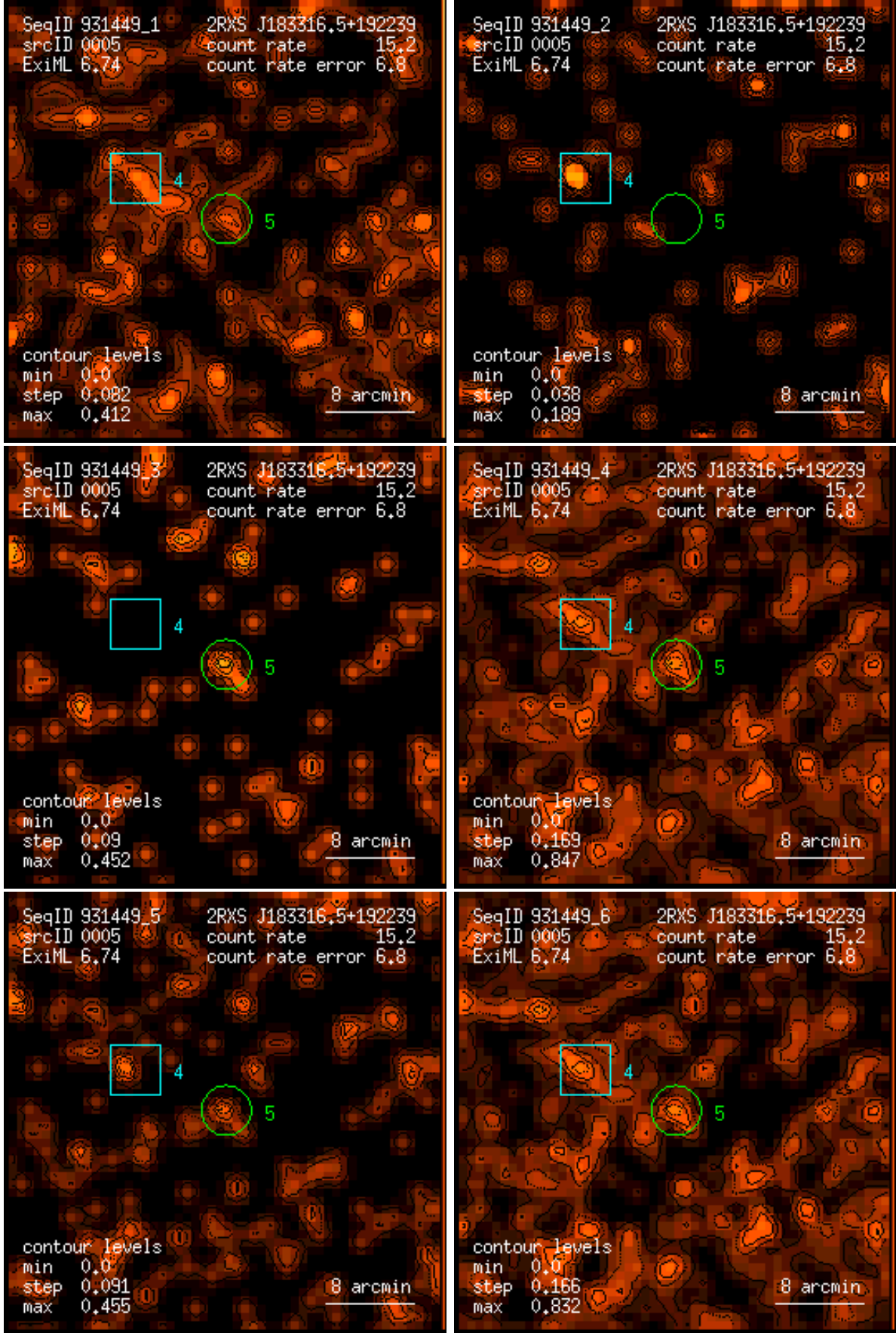
Figure 5: RASS 931449: detection 0005: band rate images, Gaussian filter: (1) PSPC channels 11 – 41, (2) 52 – 90, (3) 91 – 201, (4) 11 – 235, (5) 52 – 201, (6) 11 – 201. Broad band rates in counts/ks. Band rate contour levels in counts/ks/arcmin 2 .
