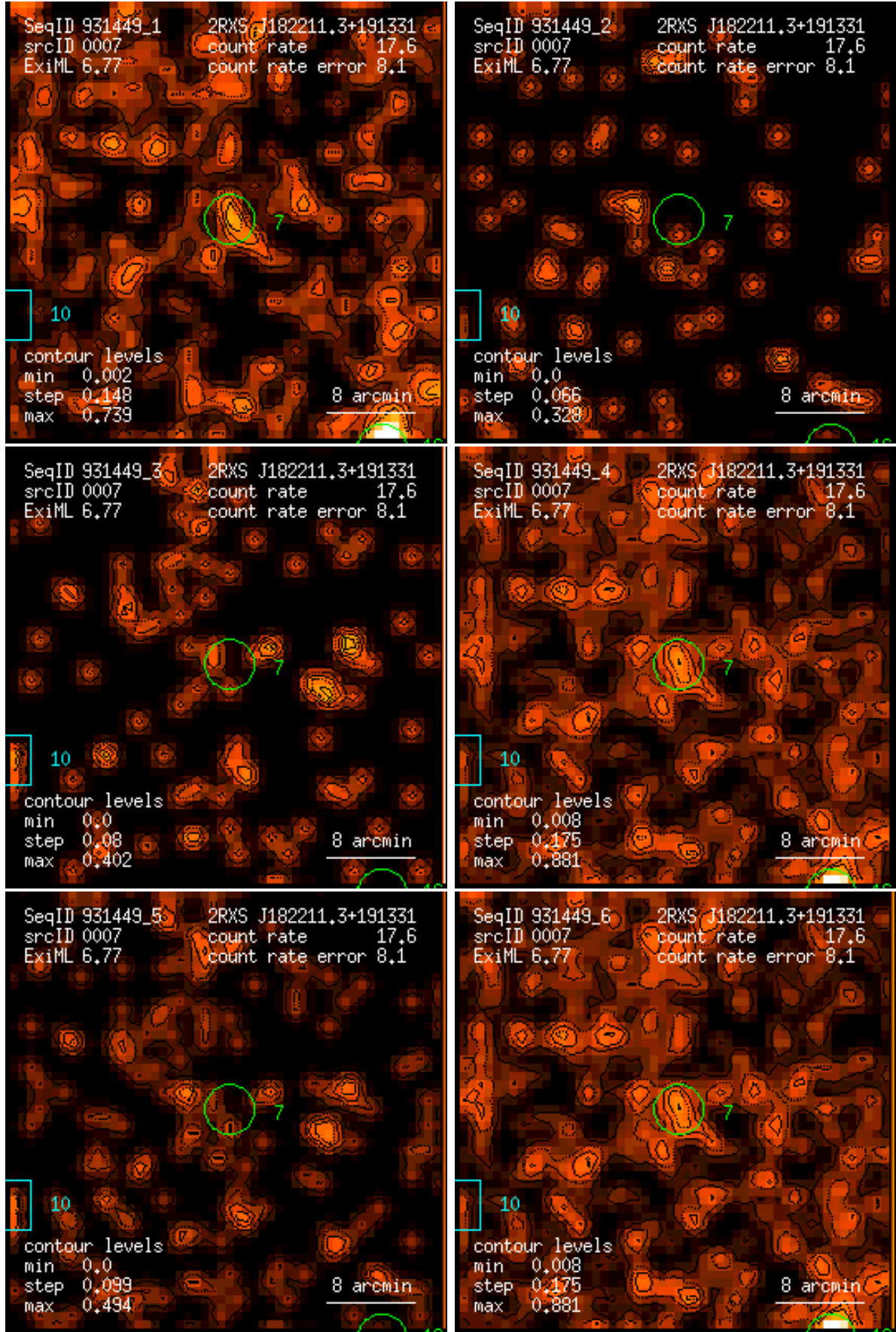
Figure 7: RASS 931449: detection 0007: band rate images, Gaussian filter: (1) PSPC channels 11 – 41, (2) 52 – 90, (3) 91 – 201, (4) 11 – 235, (5) 52 – 201, (6) 11 – 201. Broad band rates in counts/ks. Band rate contour levels in counts/ks/arcmin 2 .
