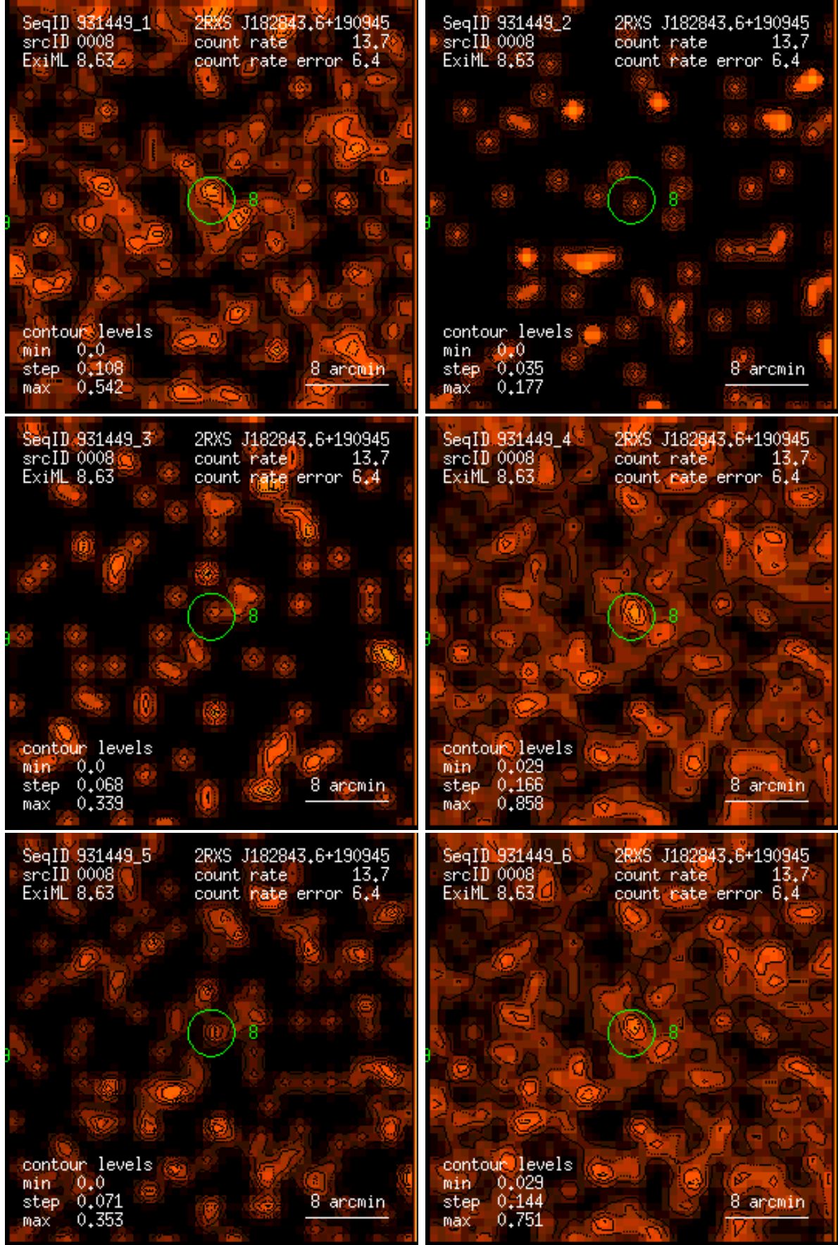
Figure 8: RASS 931449: detection 0008: band rate images, Gaussian filter: (1) PSPC channels 11 – 41, (2) 52 – 90, (3) 91 – 201, (4) 11 – 235, (5) 52 – 201, (6) 11 – 201. Broad band rates in counts/ks. Band rate contour levels in counts/ks/arcmin 2 .
