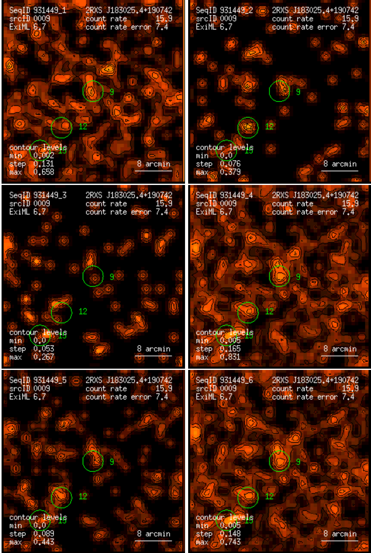
Figure 9: RASS 931449: detection 0009: band rate images, Gaussian filter: (1) PSPC channels 11 – 41, (2) 52 – 90, (3) 91 – 201, (4) 11 – 235, (5) 52 – 201, (6) 11 – 201. Broad band rates in counts/ks. Band rate contour levels in counts/ks/arcmin 2 .
