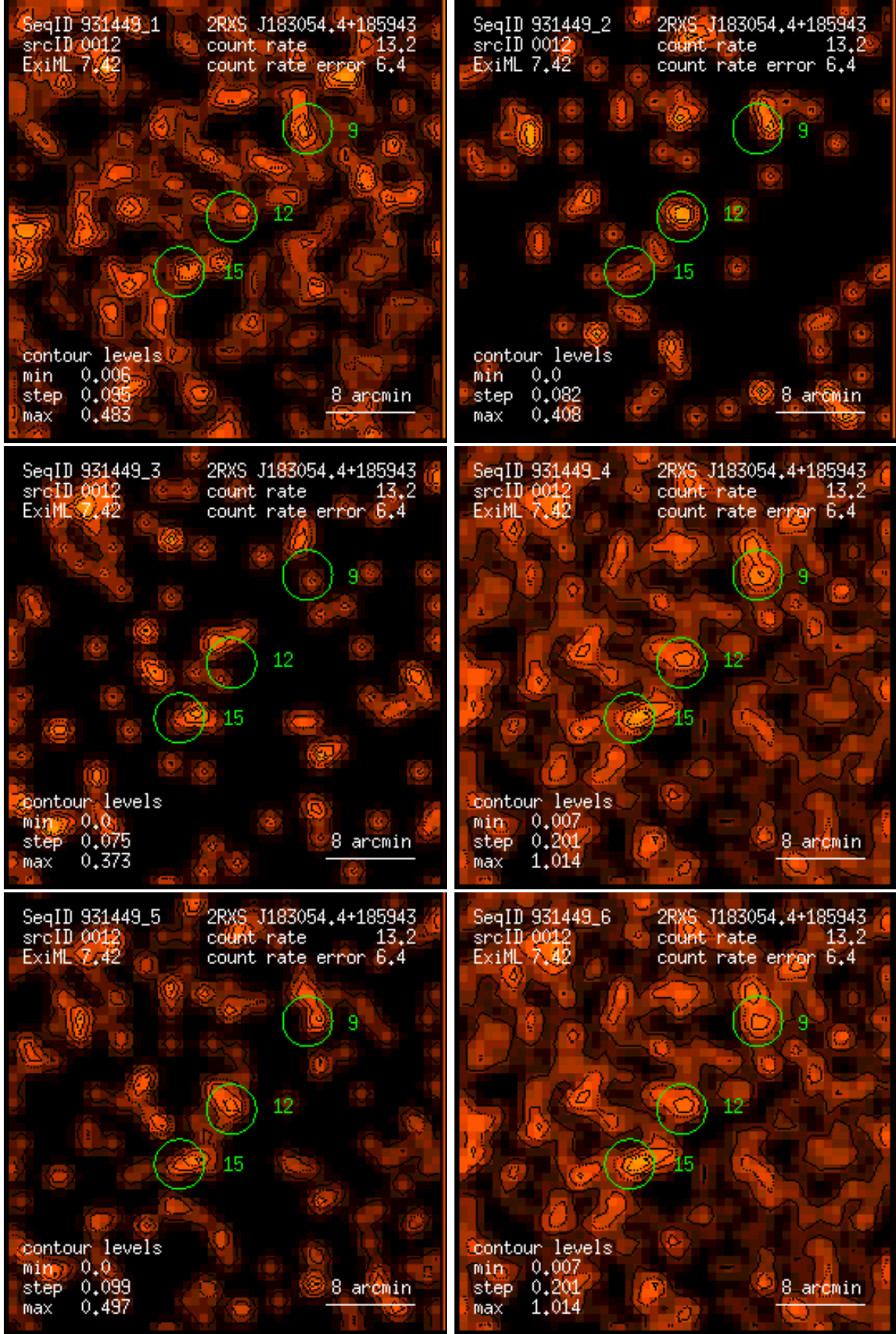
Figure 12: RASS 931449: detection 0012: band rate images, Gaussian filter: (1) PSPC channels 11 – 41, (2) 52 – 90, (3) 91 – 201, (4) 11 – 235, (5) 52 – 201, (6) 11 – 201. Broad band rates in counts/ks. Band rate contour levels in counts/ks/arcmin 2 .
