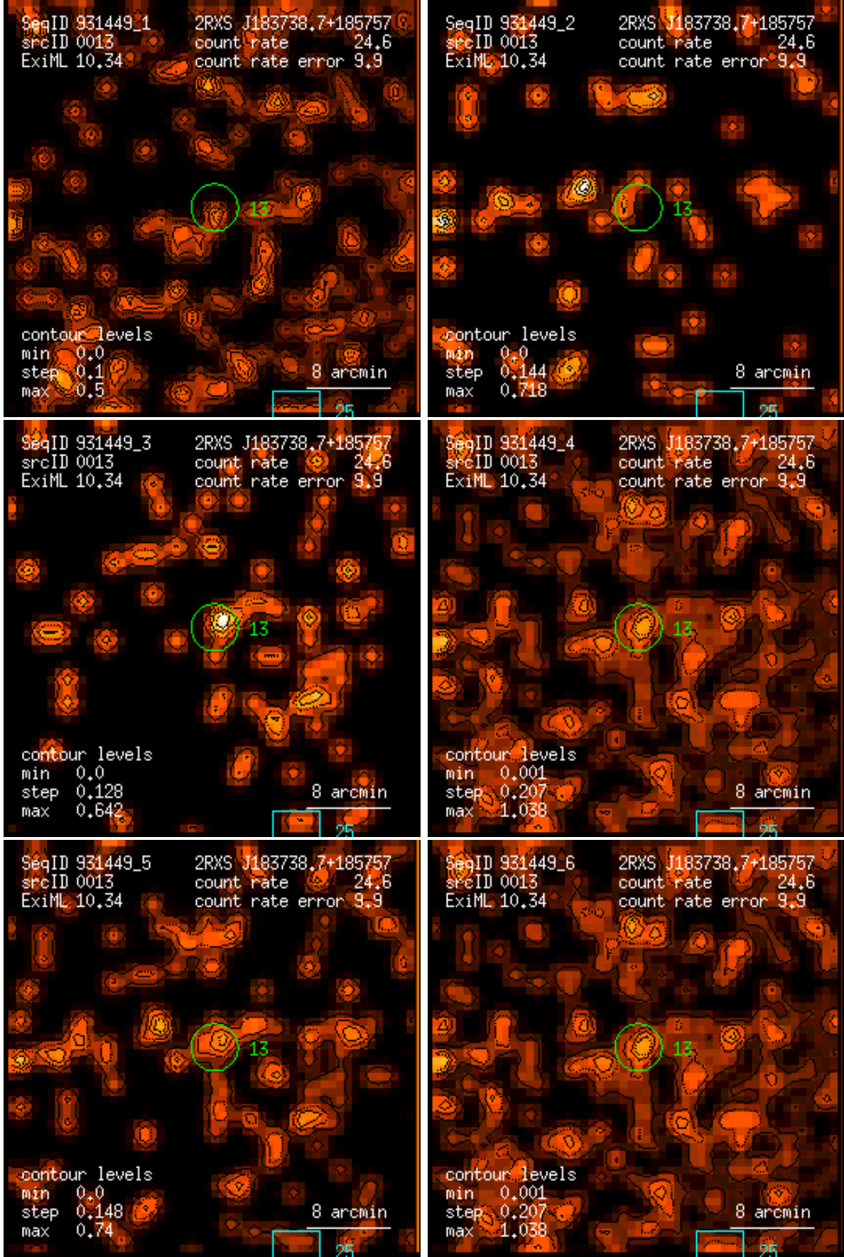
Figure 13: RASS 931449: detection 0013: band rate images, Gaussian filter: (1) PSPC channels 11 – 41, (2) 52 – 90, (3) 91 – 201, (4) 11 – 235, (5) 52 – 201, (6) 11 – 201. Broad band rates in counts/ks. Band rate contour levels in counts/ks/arcmin 2 .
