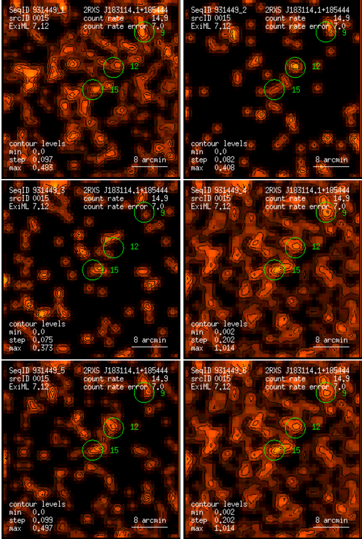
Figure 15: RASS 931449: detection 0015: band rate images, Gaussian filter: (1) PSPC channels 11 – 41, (2) 52 – 90, (3) 91 – 201, (4) 11 – 235, (5) 52 – 201, (6) 11 – 201. Broad band rates in counts/ks. Band rate contour levels in counts/ks/arcmin 2 .
