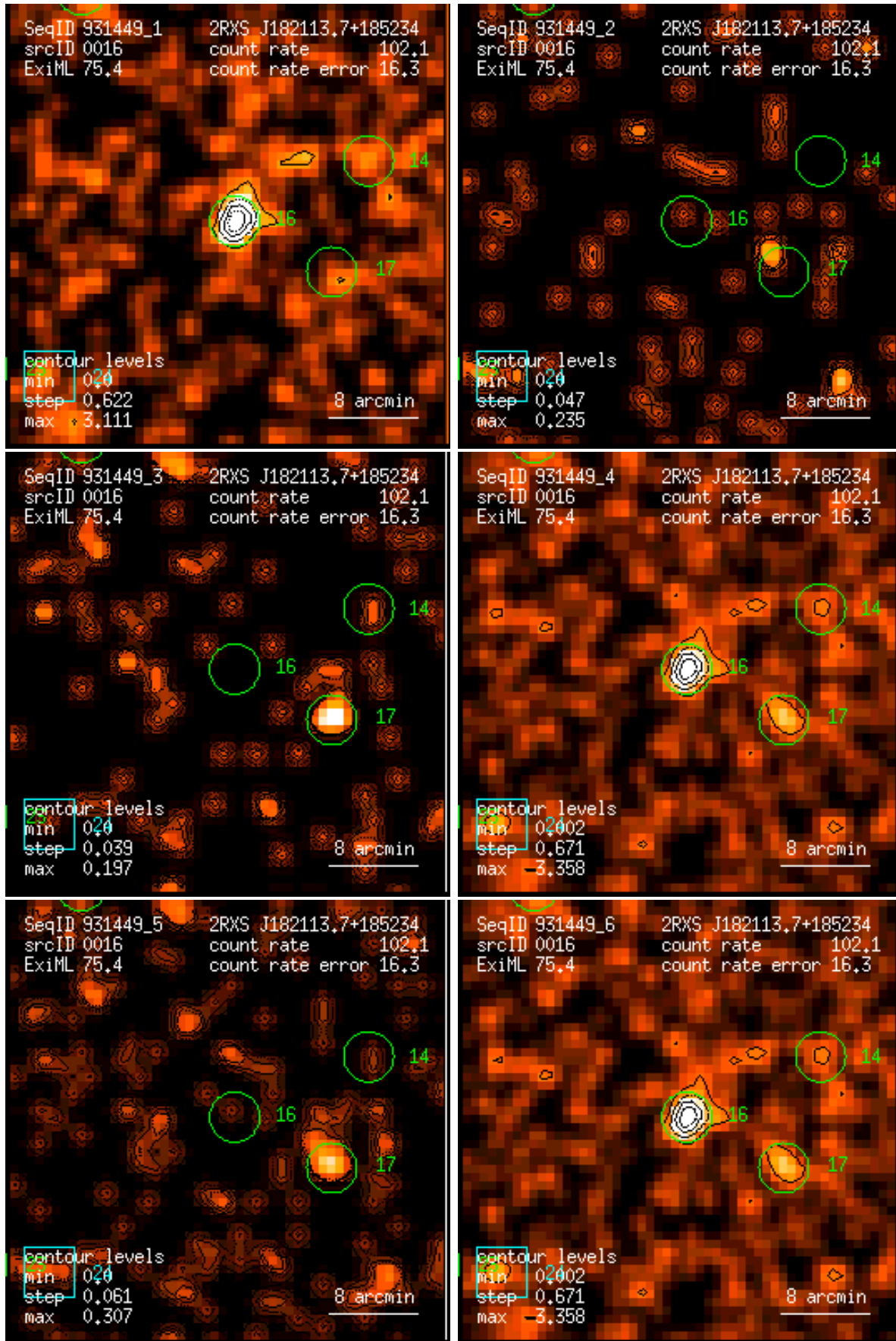
Figure 16: RASS 931449: detection 0016: band rate images, Gaussian filter: (1) PSPC channels 11 – 41, (2) 52 – 90, (3) 91 – 201, (4) 11 – 235, (5) 52 – 201, (6) 11 – 201. Broad band rates in counts/ks. Band rate contour levels in counts/ks/arcmin 2 .
