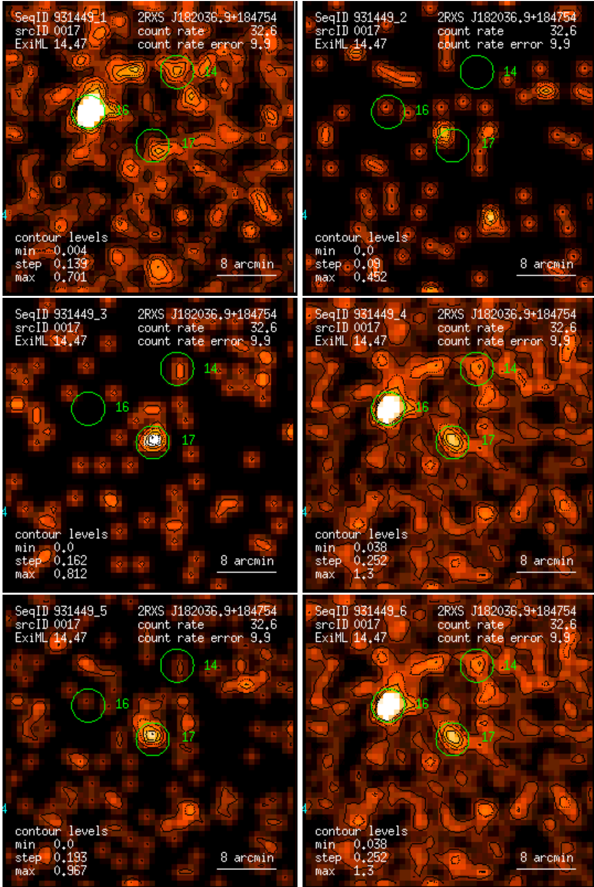
Figure 17: RASS 931449: detection 0017: band rate images, Gaussian filter: (1) PSPC channels 11 – 41, (2) 52 – 90, (3) 91 – 201, (4) 11 – 235, (5) 52 – 201, (6) 11 – 201. Broad band rates in counts/ks. Band rate contour levels in counts/ks/arcmin 2 .
