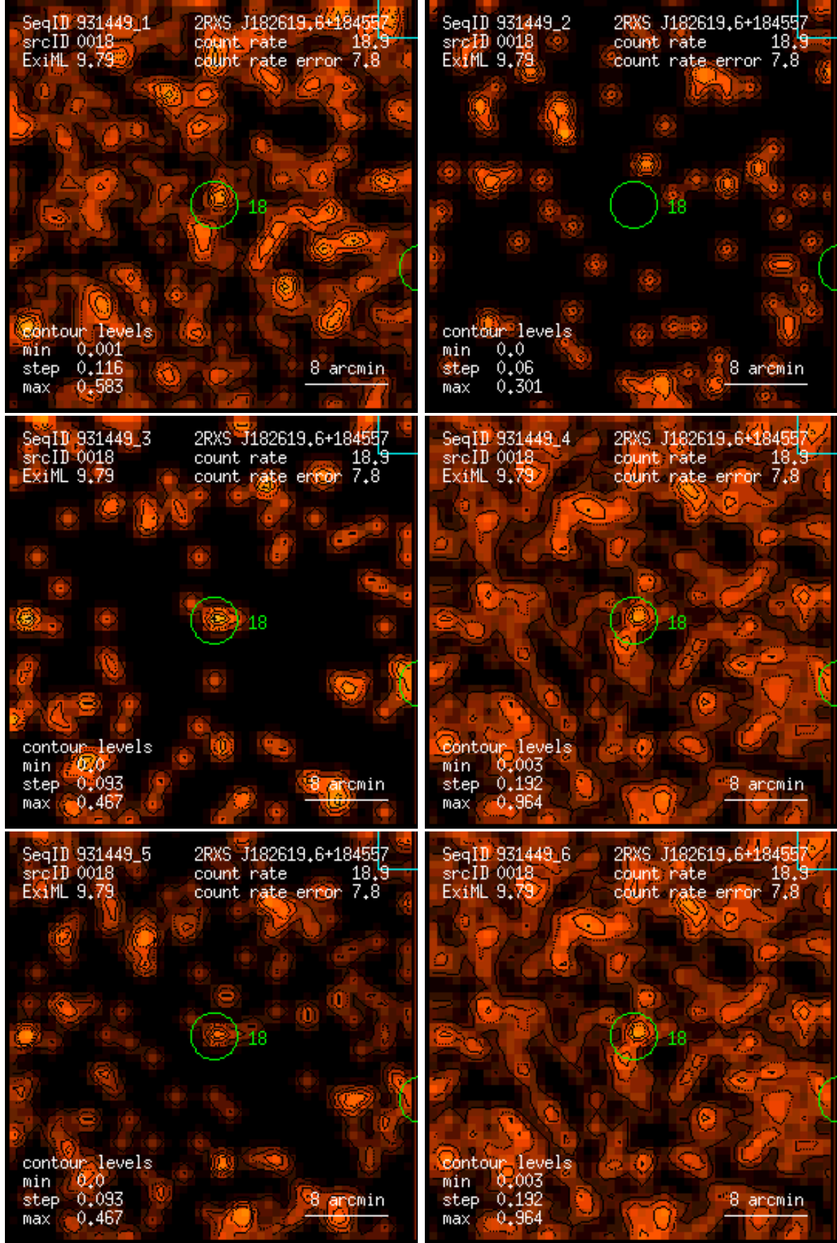
Figure 18: RASS 931449: detection 0018: band rate images, Gaussian filter: (1) PSPC channels 11 – 41, (2) 52 – 90, (3) 91 – 201, (4) 11 – 235, (5) 52 – 201, (6) 11 – 201. Broad band rates in counts/ks. Band rate contour levels in counts/ks/arcmin 2 .
