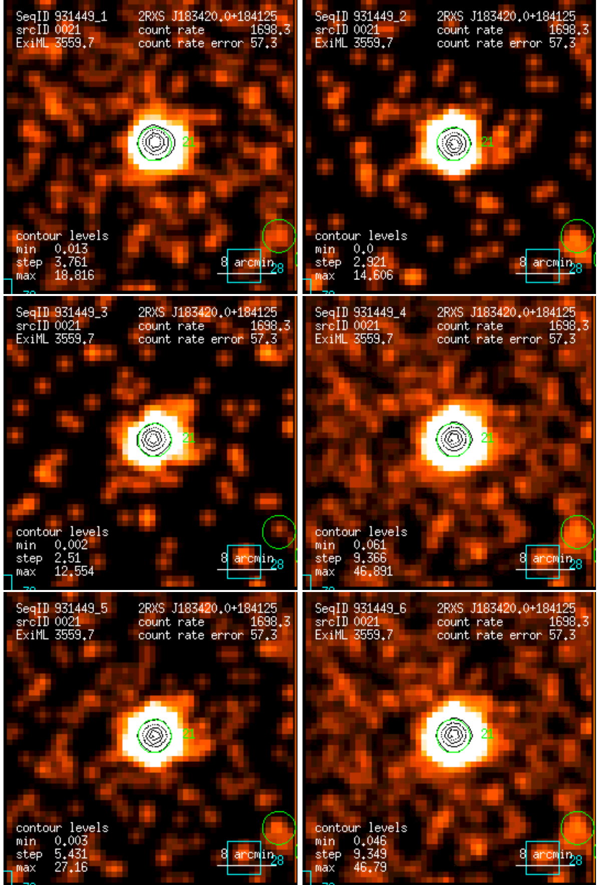
Figure 21: RASS 931449: detection 0021: band rate images, Gaussian filter: (1) PSPC channels 11 – 41, (2) 52 – 90, (3) 91 – 201, (4) 11 – 235, (5) 52 – 201, (6) 11 – 201. Broad band rates in counts/ks. Band rate contour levels in counts/ks/arcmin 2 .
