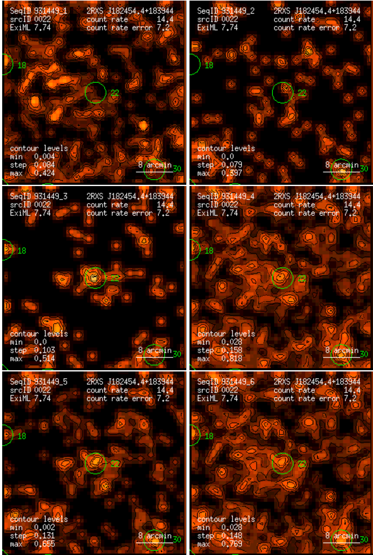
Figure 22: RASS 931449: detection 0022: band rate images, Gaussian filter: (1) PSPC channels 11 – 41, (2) 52 – 90, (3) 91 – 201, (4) 11 – 235, (5) 52 – 201, (6) 11 – 201. Broad band rates in counts/ks. Band rate contour levels in counts/ks/arcmin 2 .
