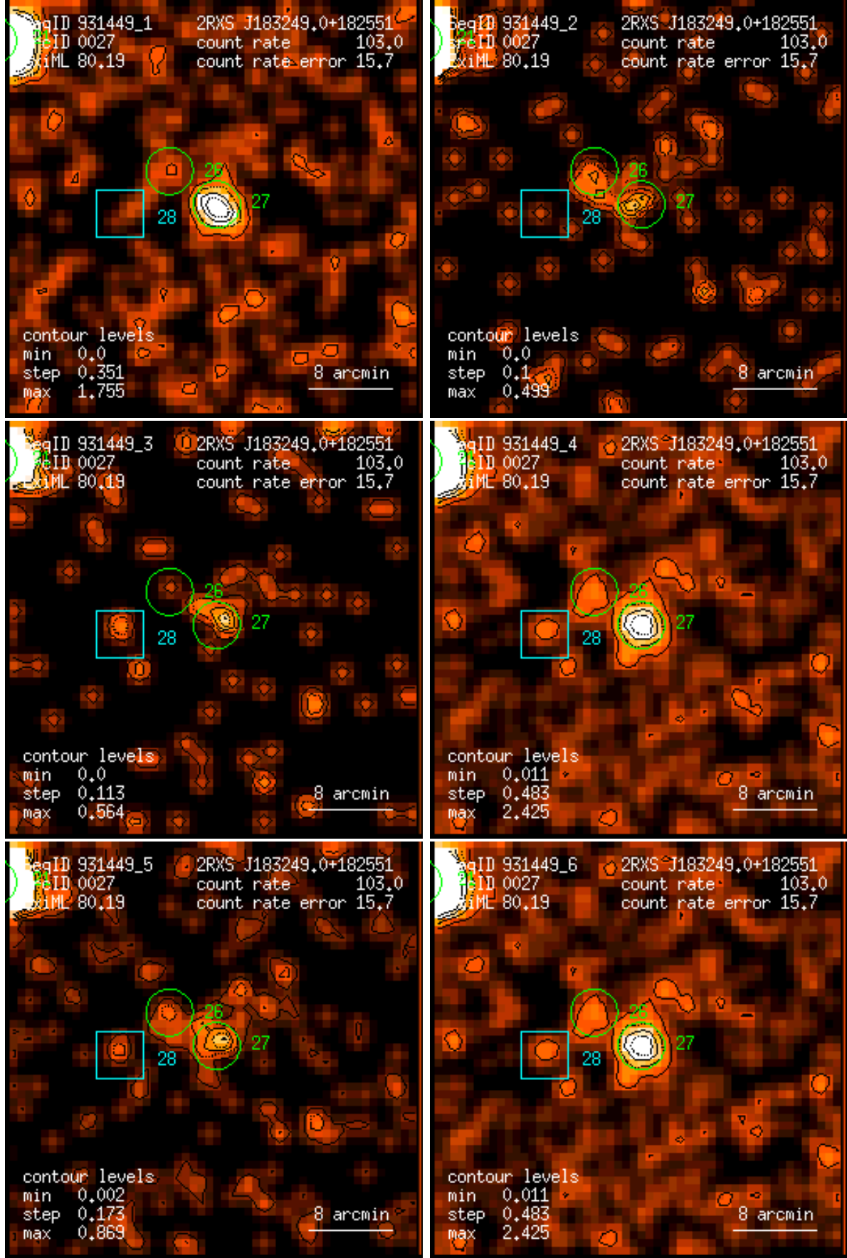
Figure 27: RASS 931449: detection 0027: band rate images, Gaussian filter: (1) PSPC channels 11 – 41, (2) 52 – 90, (3) 91 – 201, (4) 11 – 235, (5) 52 – 201, (6) 11 – 201. Broad band rates in counts/ks. Band rate contour levels in counts/ks/arcmin 2 .
