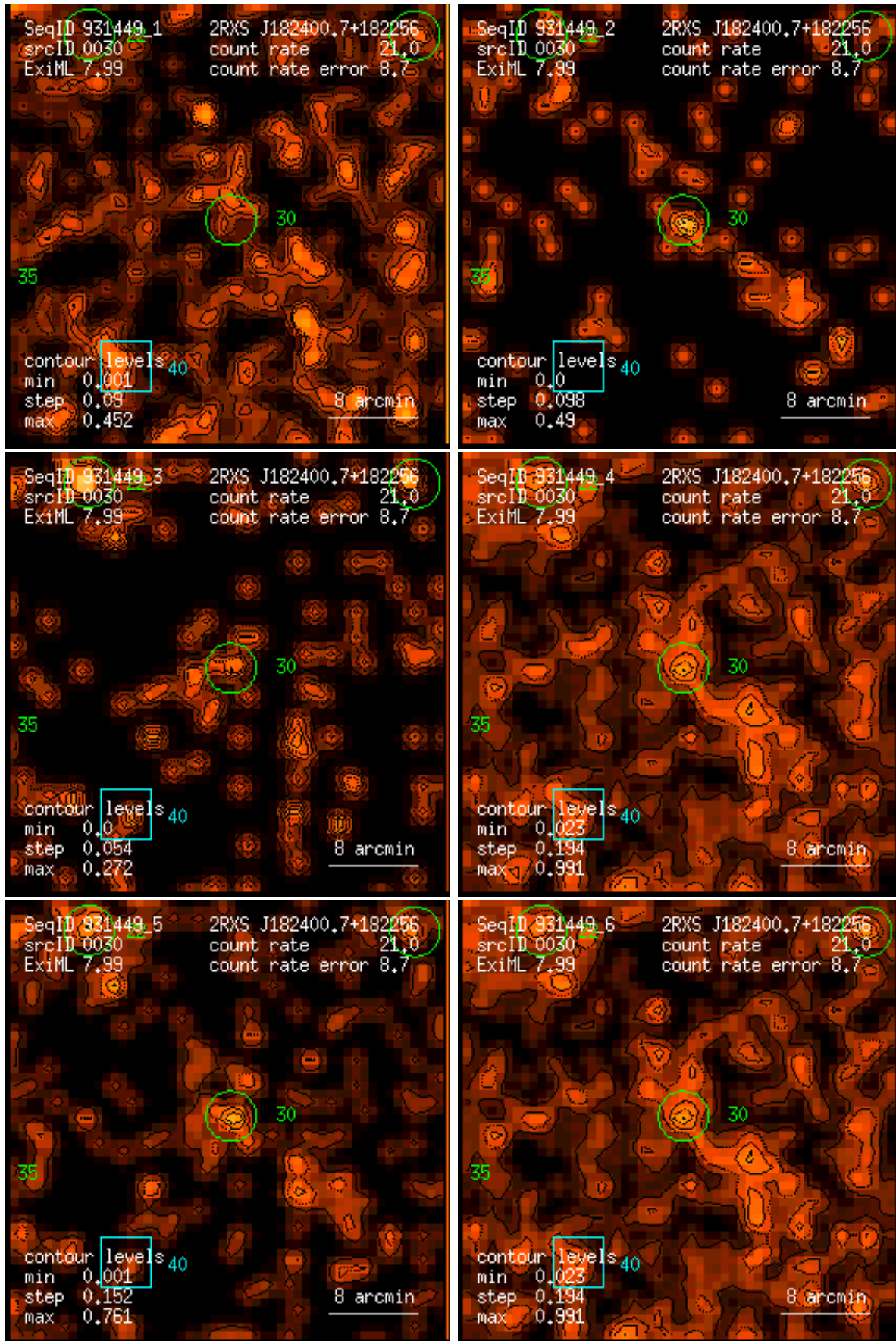
Figure 30: RASS 931449: detection 0030: band rate images, Gaussian filter: (1) PSPC channels 11 – 41, (2) 52 – 90, (3) 91 – 201, (4) 11 – 235, (5) 52 – 201, (6) 11 – 201. Broad band rates in counts/ks. Band rate contour levels in counts/ks/arcmin 2 .
