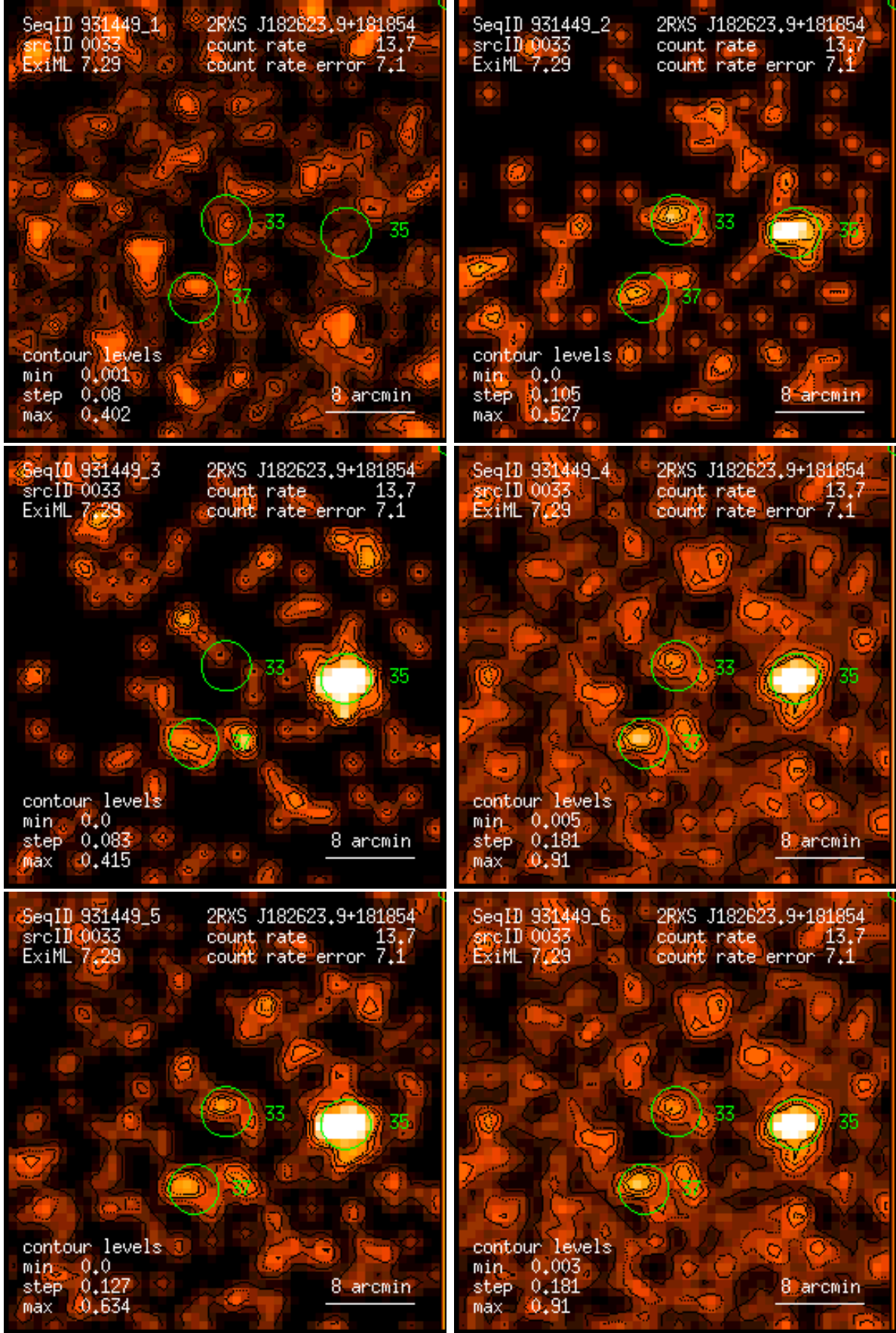
Figure 33: RASS 931449: detection 0033: band rate images, Gaussian filter: (1) PSPC channels 11 – 41, (2) 52 – 90, (3) 91 – 201, (4) 11 – 235, (5) 52 – 201, (6) 11 – 201. Broad band rates in counts/ks. Band rate contour levels in counts/ks/arcmin 2 .
