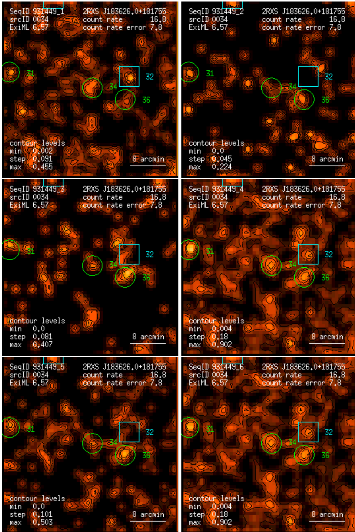
Figure 34: RASS 931449: detection 0034: band rate images, Gaussian filter: (1) PSPC channels 11 – 41, (2) 52 – 90, (3) 91 – 201, (4) 11 – 235, (5) 52 – 201, (6) 11 – 201. Broad band rates in counts/ks. Band rate contour levels in counts/ks/arcmin 2 .
