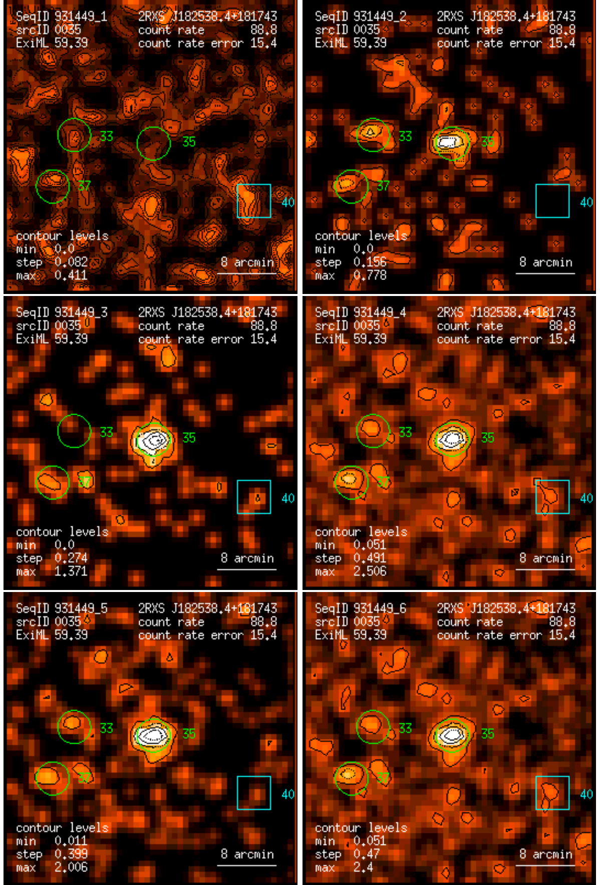
Figure 35: RASS 931449: detection 0035: band rate images, Gaussian filter: (1) PSPC channels 11 – 41, (2) 52 – 90, (3) 91 – 201, (4) 11 – 235, (5) 52 – 201, (6) 11 – 201. Broad band rates in counts/ks. Band rate contour levels in counts/ks/arcmin 2 .
