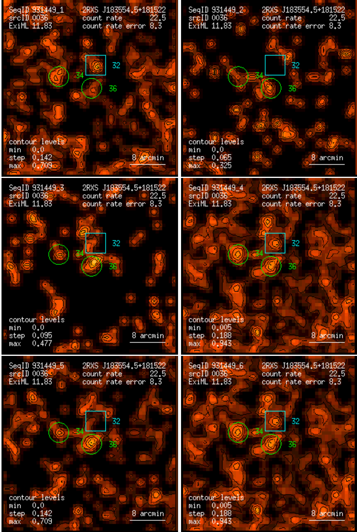
Figure 36: RASS 931449: detection 0036: band rate images, Gaussian filter: (1) PSPC channels 11 – 41, (2) 52 – 90, (3) 91 – 201, (4) 11 – 235, (5) 52 – 201, (6) 11 – 201. Broad band rates in counts/ks. Band rate contour levels in counts/ks/arcmin 2 .
