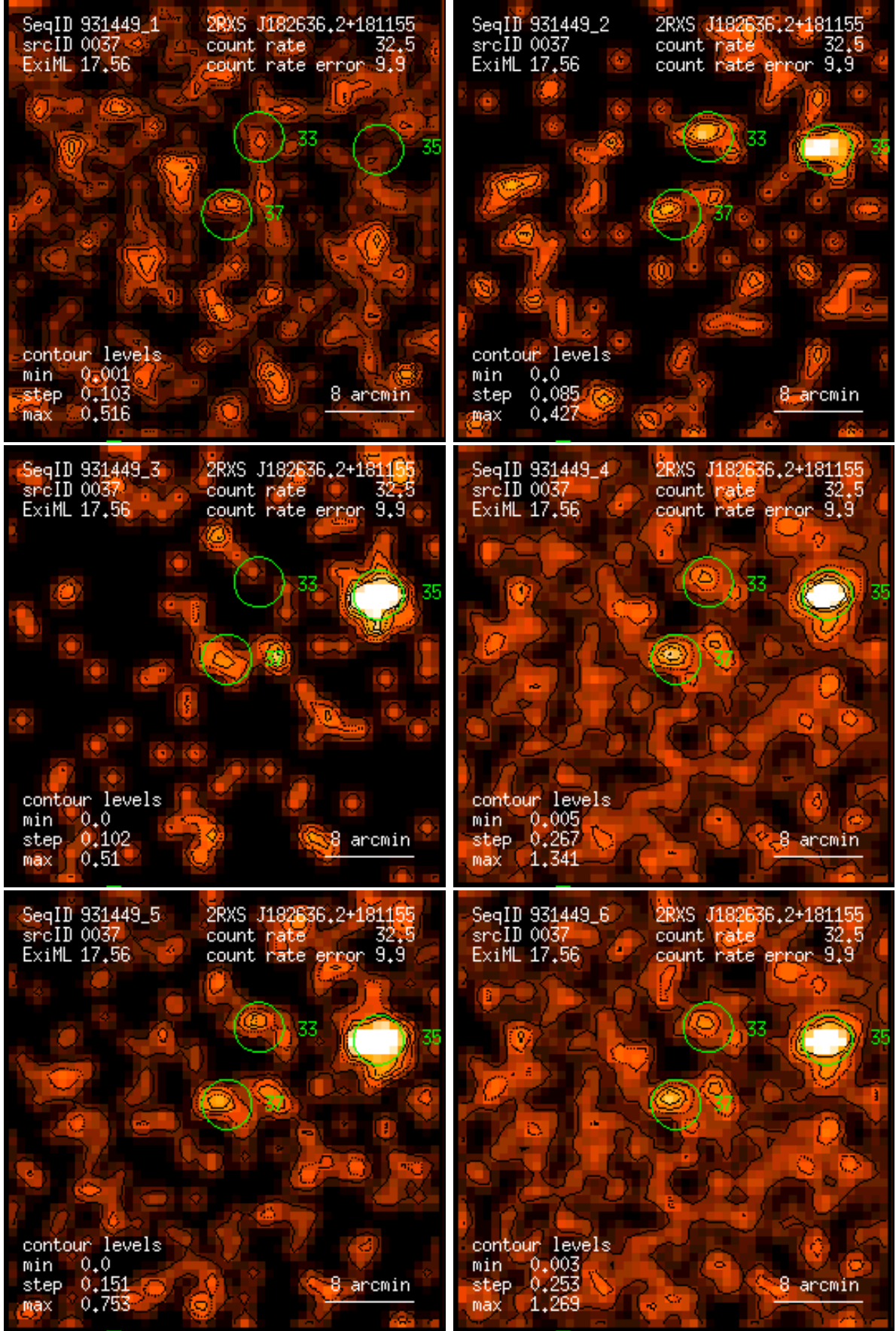
Figure 37: RASS 931449: detection 0037: band rate images, Gaussian filter: (1) PSPC channels 11 – 41, (2) 52 – 90, (3) 91 – 201, (4) 11 – 235, (5) 52 – 201, (6) 11 – 201. Broad band rates in counts/ks. Band rate contour levels in counts/ks/arcmin 2 .
