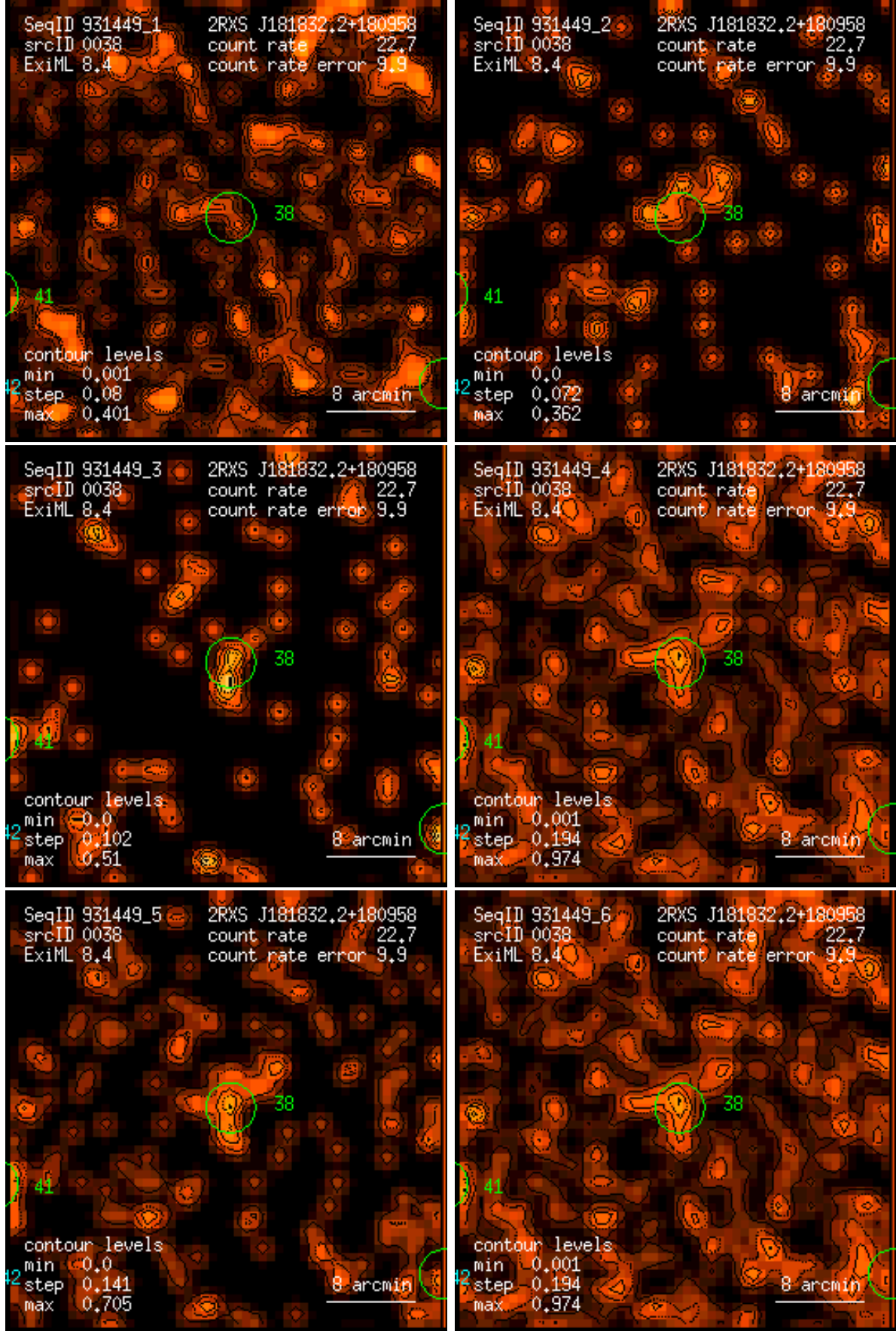
Figure 38: RASS 931449: detection 0038: band rate images, Gaussian filter: (1) PSPC channels 11 – 41, (2) 52 – 90, (3) 91 – 201, (4) 11 – 235, (5) 52 – 201, (6) 11 – 201. Broad band rates in counts/ks. Band rate contour levels in counts/ks/arcmin 2 .
