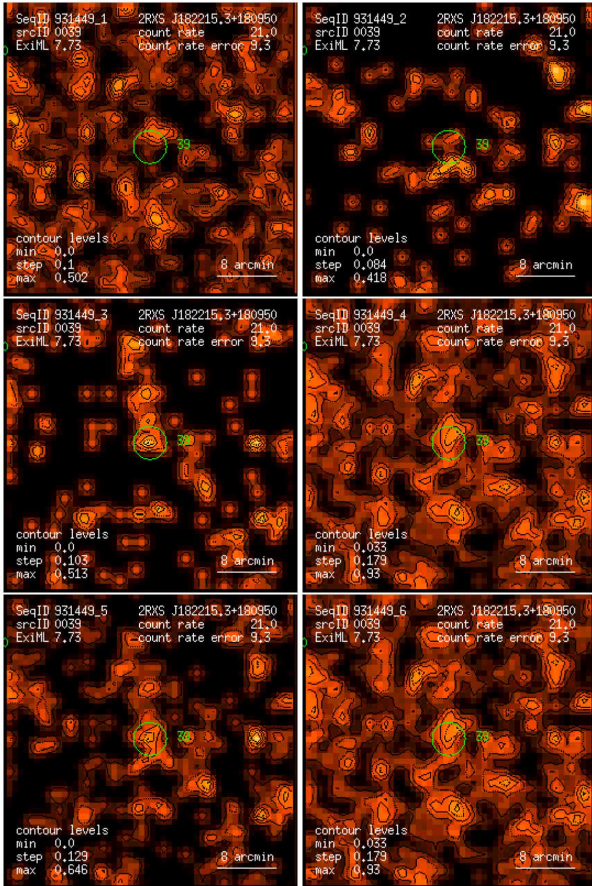
Figure 39: RASS 931449: detection 0039: band rate images, Gaussian filter: (1) PSPC channels 11 – 41, (2) 52 – 90, (3) 91 – 201, (4) 11 – 235, (5) 52 – 201, (6) 11 – 201. Broad band rates in counts/ks. Band rate contour levels in counts/ks/arcmin 2 .
