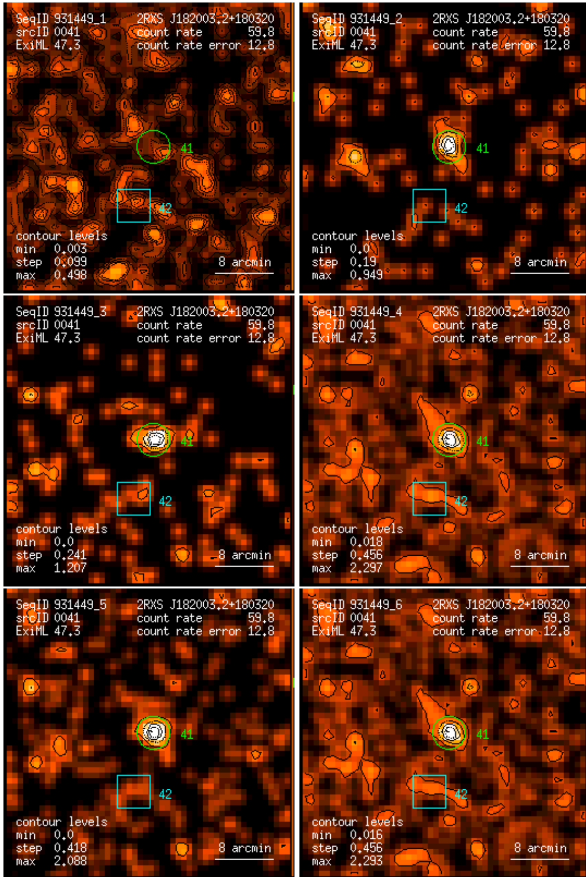
Figure 41: RASS 931449: detection 0041: band rate images, Gaussian filter: (1) PSPC channels 11 – 41, (2) 52 – 90, (3) 91 – 201, (4) 11 – 235, (5) 52 – 201, (6) 11 – 201. Broad band rates in counts/ks. Band rate contour levels in counts/ks/arcmin 2 .
