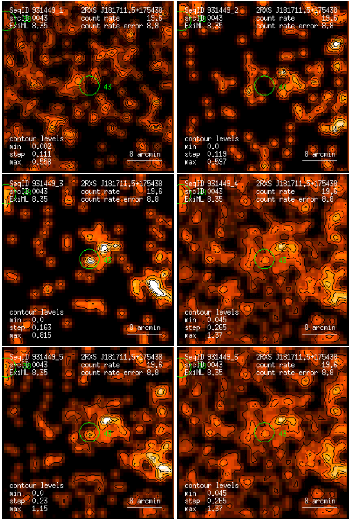
Figure 43: RASS 931449: detection 0043: band rate images, Gaussian filter: (1) PSPC channels 11 – 41, (2) 52 – 90, (3) 91 – 201, (4) 11 – 235, (5) 52 – 201, (6) 11 – 201. Broad band rates in counts/ks. Band rate contour levels in counts/ks/arcmin 2 .
