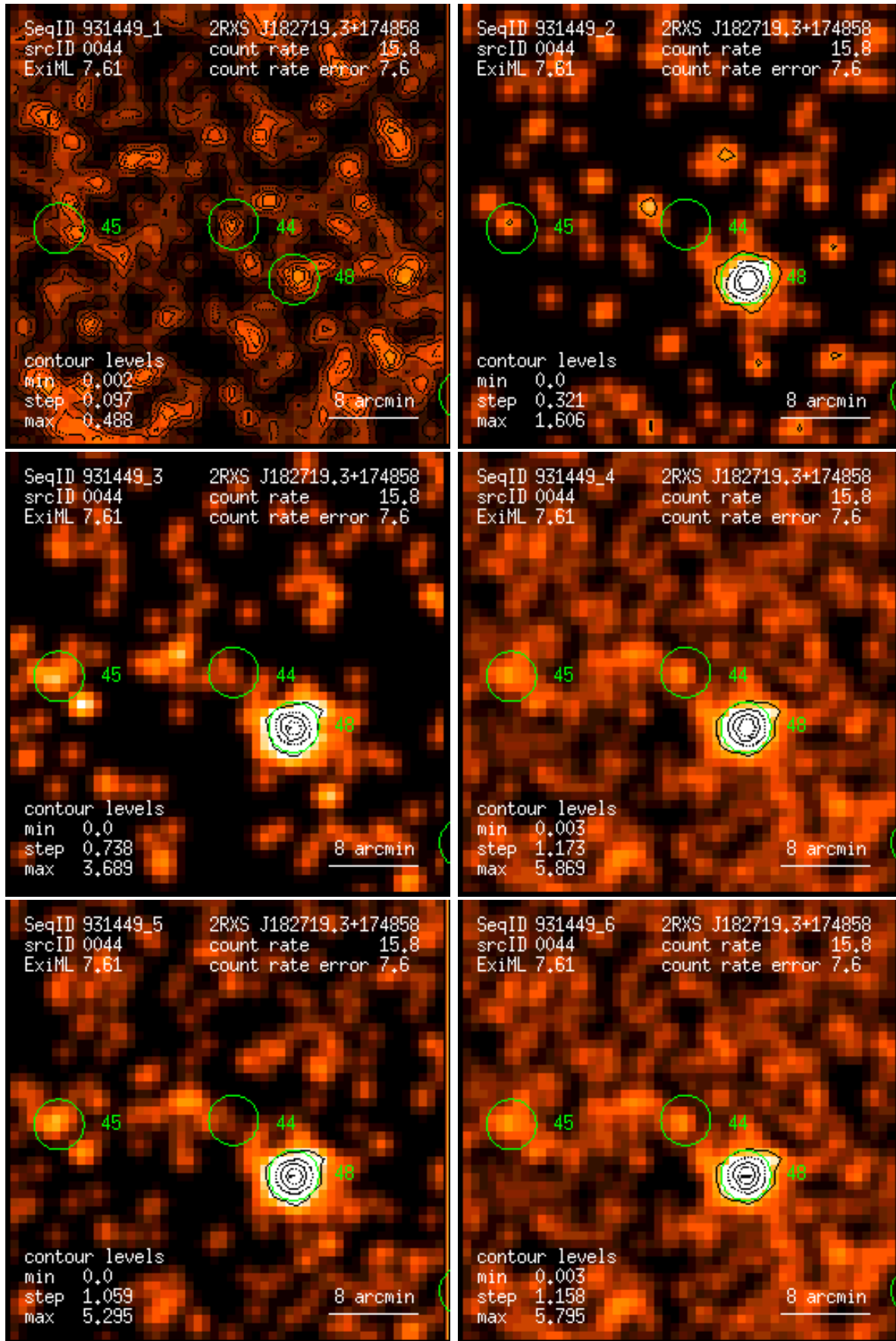
Figure 44: RASS 931449: detection 0044: band rate images, Gaussian filter: (1) PSPC channels 11 – 41, (2) 52 – 90, (3) 91 – 201, (4) 11 – 235, (5) 52 – 201, (6) 11 – 201. Broad band rates in counts/ks. Band rate contour levels in counts/ks/arcmin 2 .
