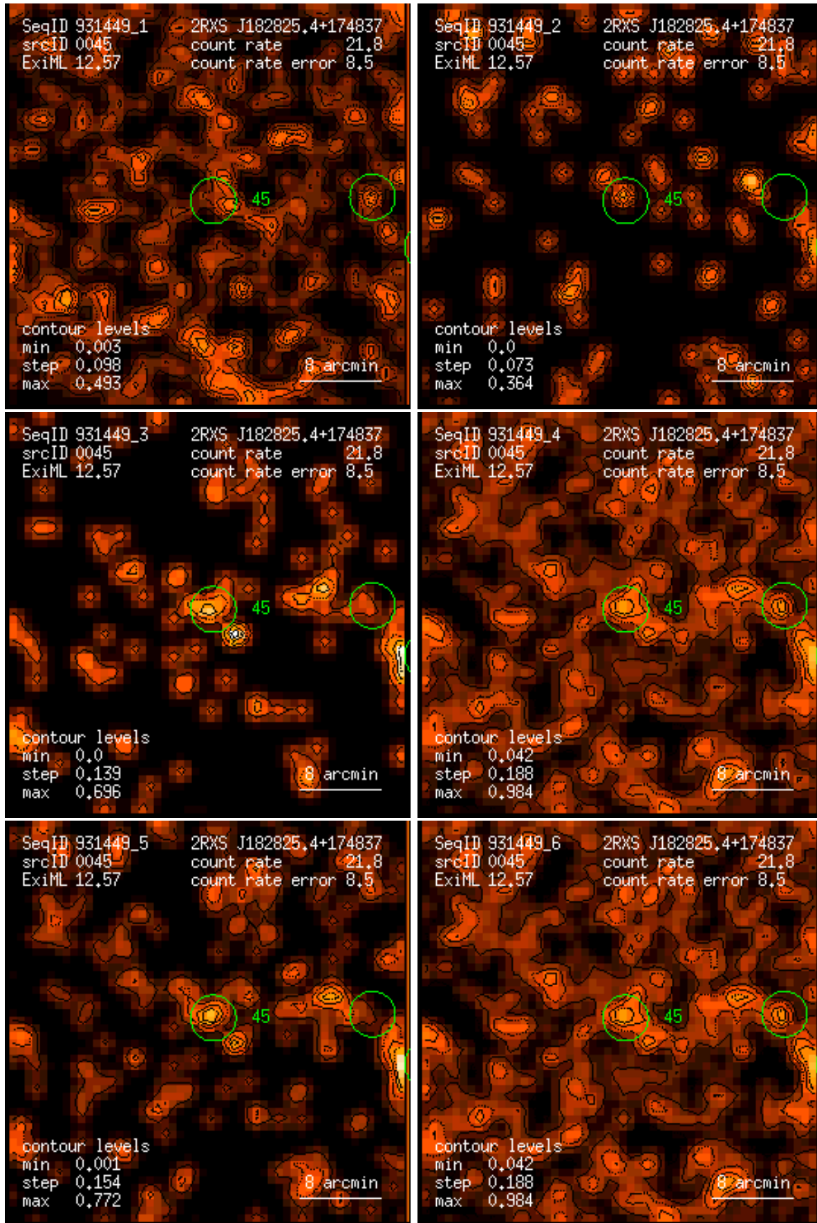
Figure 45: RASS 931449: detection 0045: band rate images, Gaussian filter: (1) PSPC channels 11 – 41, (2) 52 – 90, (3) 91 – 201, (4) 11 – 235, (5) 52 – 201, (6) 11 – 201. Broad band rates in counts/ks. Band rate contour levels in counts/ks/arcmin 2 .
