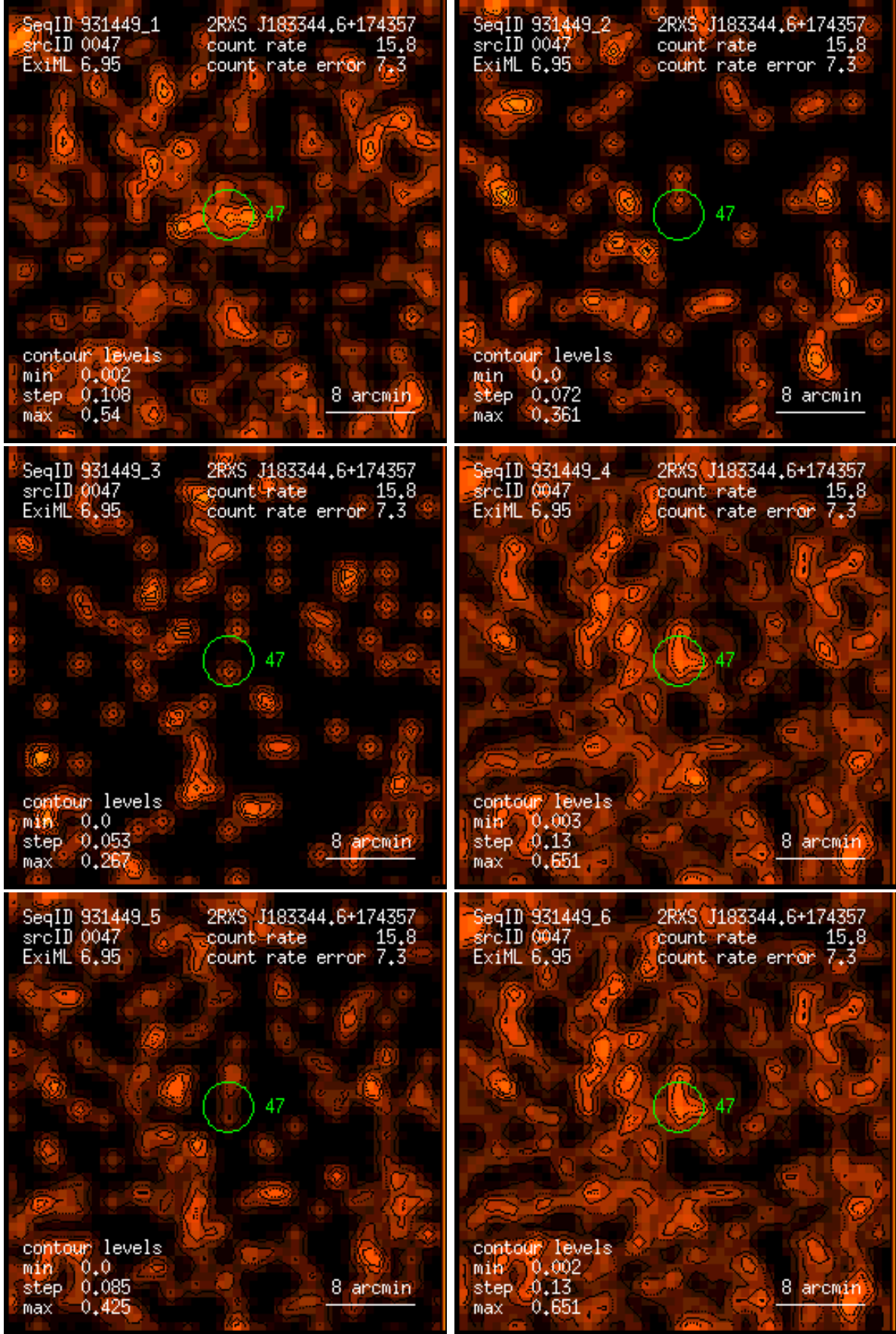
Figure 47: RASS 931449: detection 0047: band rate images, Gaussian filter: (1) PSPC channels 11 – 41, (2) 52 – 90, (3) 91 – 201, (4) 11 – 235, (5) 52 – 201, (6) 11 – 201. Broad band rates in counts/ks. Band rate contour levels in counts/ks/arcmin 2 .
