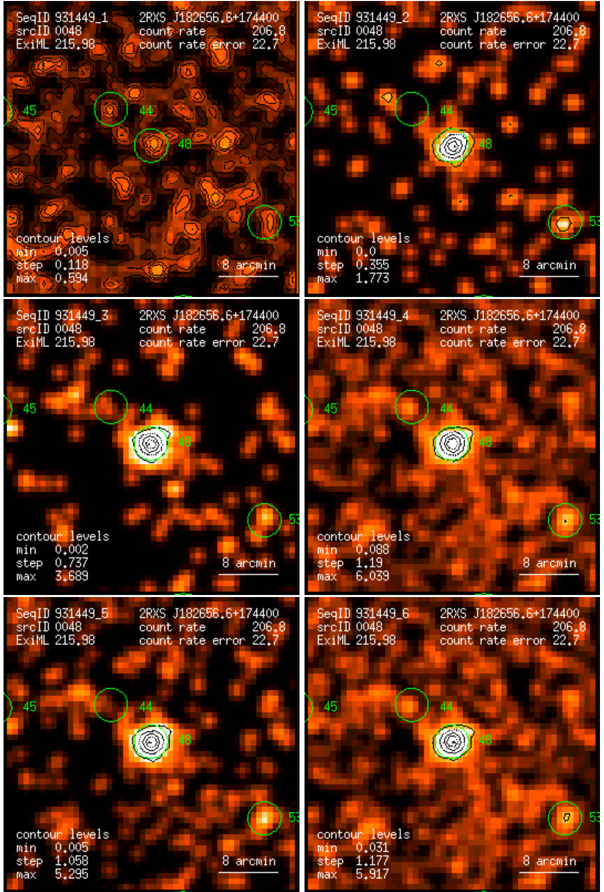
Figure 48: RASS 931449: detection 0048: band rate images, Gaussian filter: (1) PSPC channels 11 – 41, (2) 52 – 90, (3) 91 – 201, (4) 11 – 235, (5) 52 – 201, (6) 11 – 201. Broad band rates in counts/ks. Band rate contour levels in counts/ks/arcmin 2 .
