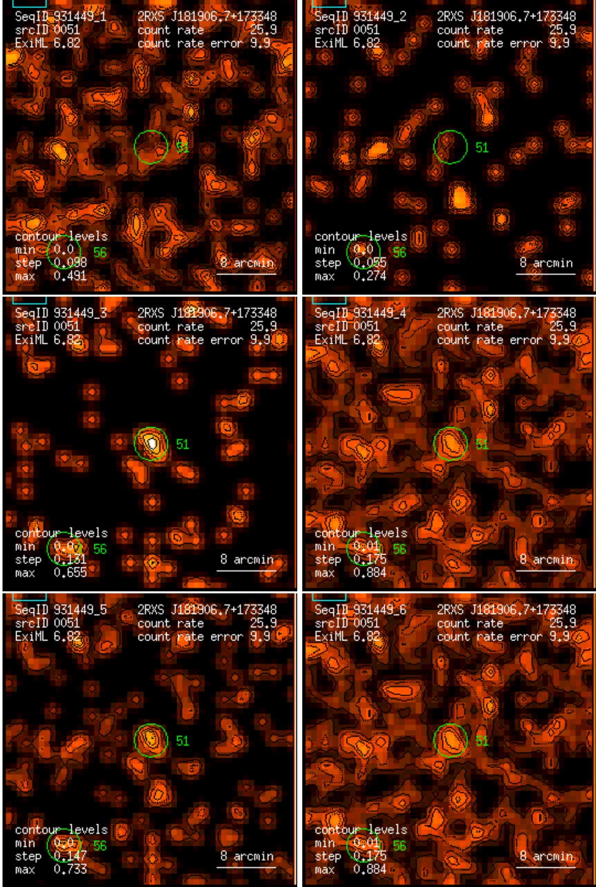
Figure 51: RASS 931449: detection 0051: band rate images, Gaussian filter: (1) PSPC channels 11 – 41, (2) 52 – 90, (3) 91 – 201, (4) 11 – 235, (5) 52 – 201, (6) 11 – 201. Broad band rates in counts/ks. Band rate contour levels in counts/ks/arcmin 2 .
