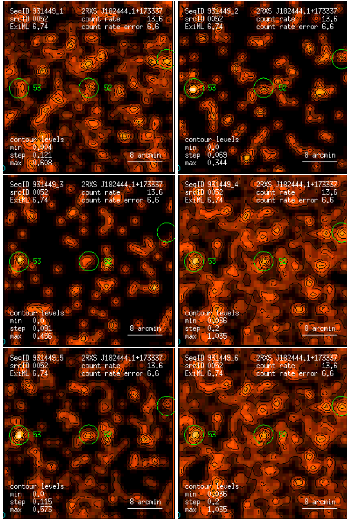
Figure 52: RASS 931449: detection 0052: band rate images, Gaussian filter: (1) PSPC channels 11 – 41, (2) 52 – 90, (3) 91 – 201, (4) 11 – 235, (5) 52 – 201, (6) 11 – 201. Broad band rates in counts/ks. Band rate contour levels in counts/ks/arcmin 2 .
