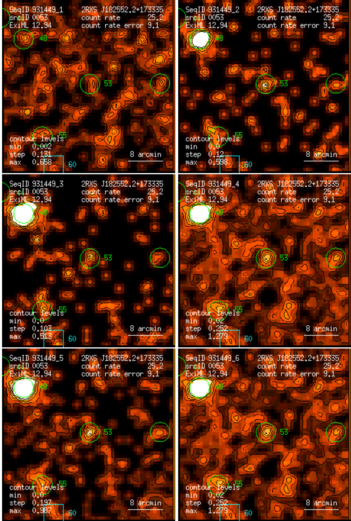
Figure 53: RASS 931449: detection 0053: band rate images, Gaussian filter: (1) PSPC channels 11 – 41, (2) 52 – 90, (3) 91 – 201, (4) 11 – 235, (5) 52 – 201, (6) 11 – 201. Broad band rates in counts/ks. Band rate contour levels in counts/ks/arcmin 2 .
