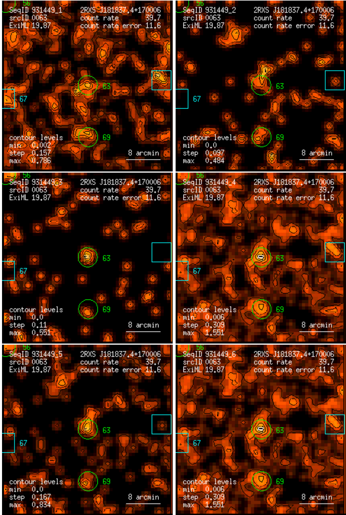
Figure 63: RASS 931449: detection 0063: band rate images, Gaussian filter: (1) PSPC channels 11 – 41, (2) 52 – 90, (3) 91 – 201, (4) 11 – 235, (5) 52 – 201, (6) 11 – 201. Broad band rates in counts/ks. Band rate contour levels in counts/ks/arcmin 2 .
