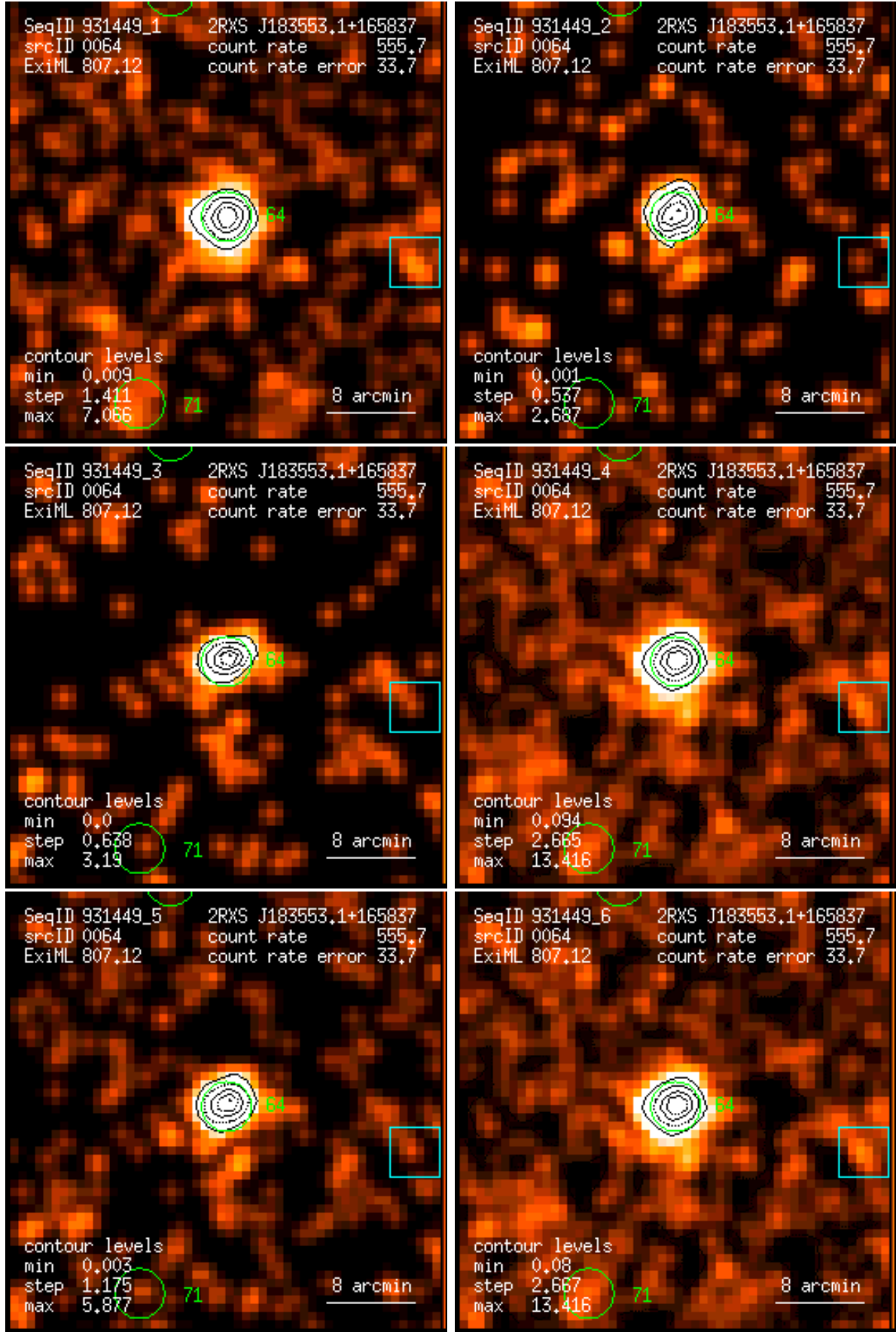
Figure 64: RASS 931449: detection 0064: band rate images, Gaussian filter: (1) PSPC channels 11 – 41, (2) 52 – 90, (3) 91 – 201, (4) 11 – 235, (5) 52 – 201, (6) 11 – 201. Broad band rates in counts/ks. Band rate contour levels in counts/ks/arcmin 2 .
