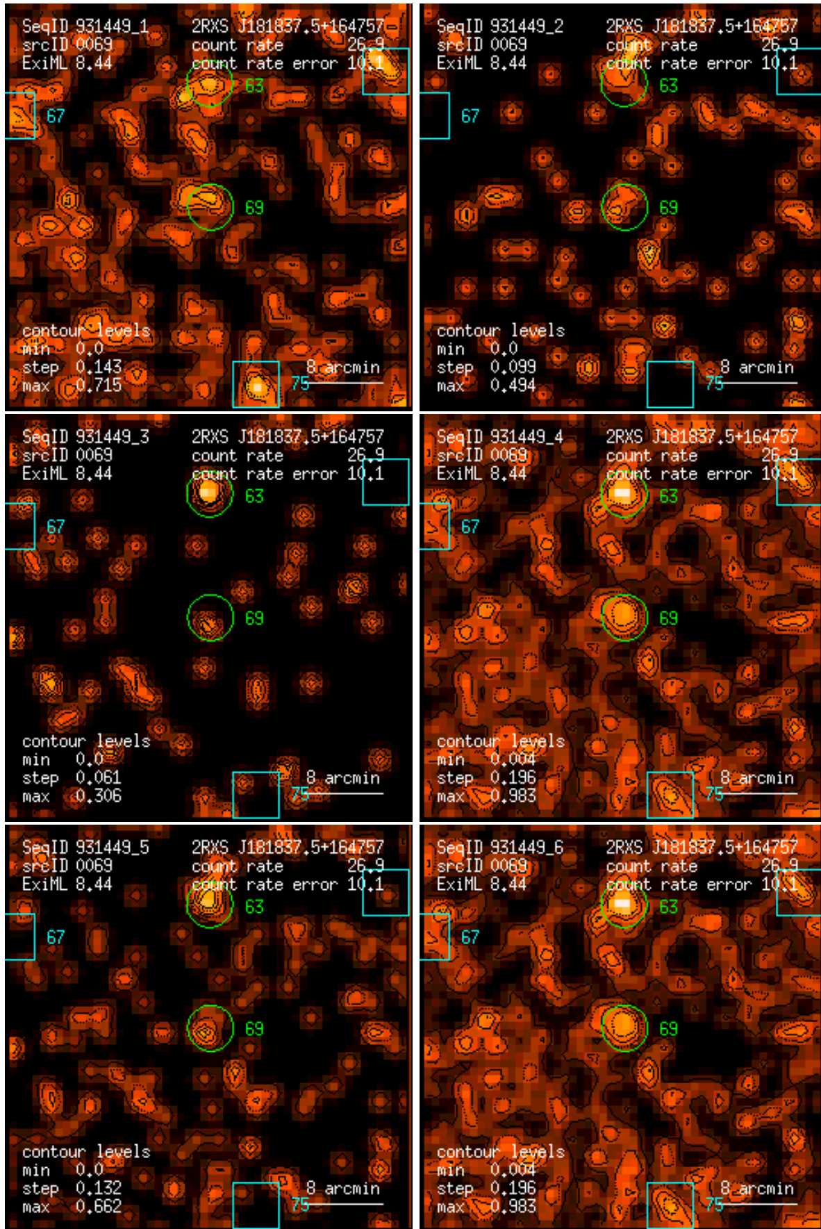
Figure 69: RASS 931449: detection 0069: band rate images, Gaussian filter: (1) PSPC channels 11 – 41, (2) 52 – 90, (3) 91 – 201, (4) 11 – 235, (5) 52 – 201, (6) 11 – 201. Broad band rates in counts/ks. Band rate contour levels in counts/ks/arcmin 2 .
